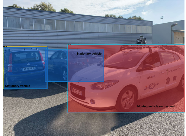
Fig. 1. Semantic-guided RANSAC scheme applied for moving object detection in the campus of École Centrale de Nantes, blue color stands for stationary objects and red color represents non-stationary objects
