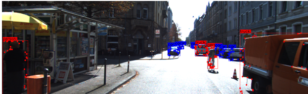
Fig. 5. Flow vector bound constraint for detecting moving objects with degenerate motion with the frame from KITTI raw data sequence 05
