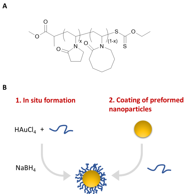
Scheme 1. A) Structure of copolymer and B) the two synthetic pathways used for the formation of nanohybrids ( in situ formation and coating of preformed nanoparticles).
