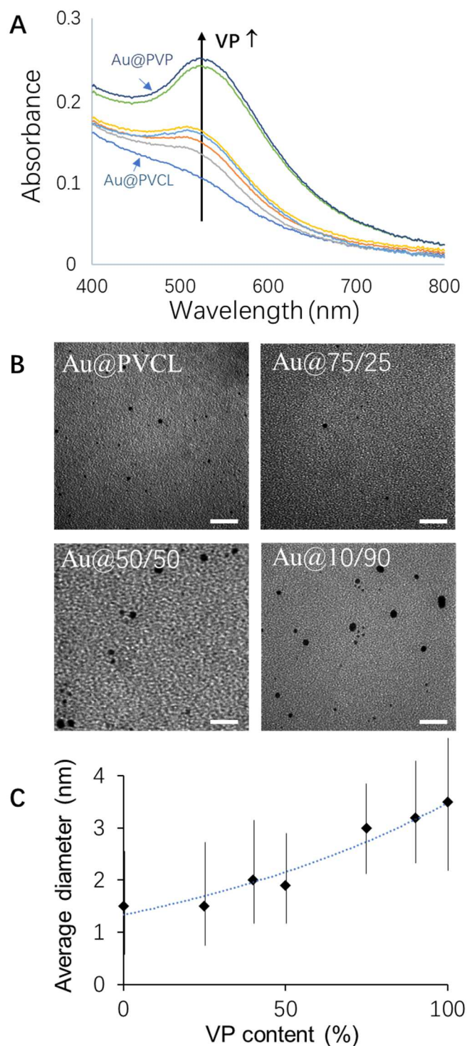
Fig. 1. In situ formation of AuNPs in presence of P(VCL/VP) 20k with [Au^0] = 5 \times 10^{-4} mol·L -1 and [polymer] = 10 -2 wt.%. A) Changes in absorption spectra as a function of the VP content within the polymer (increasing from 0, 25, 40, 50, 75, 90 and 100 %) observed 5 days after NPs formation. B) TEM images for Au@PVCL, Au@75/25, Au@50/50 and Au@10/90 and C) Evolution of average size as a function of VP content (the line is only a guide for the eyes).
