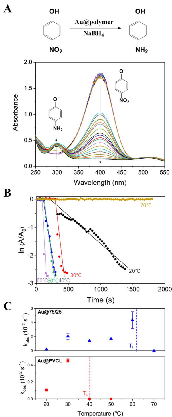
Fig. 4. A) UV-vis spectra of the reduction of p -nitrophenol to p -aminophenol by \text{NaBH}_4 catalysed by Au@75/25 at 20 °C. B) Plots of \ln(A/A_0) vs time for Au@75/25 at different temperatures and C) pseudo-first order kinetic constant ( k_{\text{obs}} ) as a function of temperature for Au@PVCL and Au@75/25 (the blue and red lines are only a guide for the eyes) ( [p\text{-nitrophenol}] = 10^{-4} \text{ mol}\cdot\text{L}^{-1} , [\text{Au}^0] = 5\times 10^{-5} \text{ mol}\cdot\text{L}^{-1} , [\text{NaBH}_4] = 3\times 10^{-3} \text{ mol}\cdot\text{L}^{-1} , [\text{polymer}] = 5\times 10^{-3} \text{ wt.}\% ).
