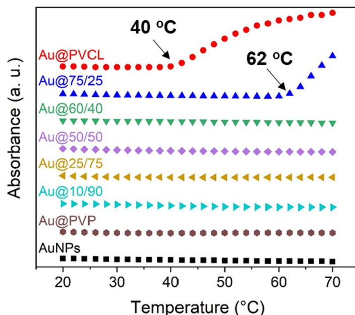
Fig. 3. Evolution of absorbance (an arbitrary unit was chosen) at 520 nm as a function of temperature for pristine AuNPs and AuNPs covered by different polymers ( [\text{polymer}] = 2.5 \times 10^{-2} \text{ wt.}\% and [\text{Au}^0] = 2.5 \times 10^{-4} \text{ mol}\cdot\text{L}^{-1} ).
