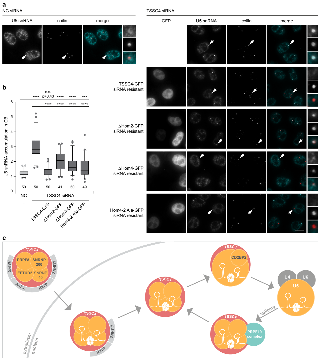
Fig. 8 Hom2 and Hom4 regions are important for TSSC4 function in tri-snRNP formation. a TSSC4 was downregulated by siRNA followed by expression of siRNA-resistant WT TSSC4-GFP, ΔHom2-GFP, ΔHom4-GFP, and Hom4-2 Ala -GFP constructs. Tri-snRNP formation was assayed by U5 snRNA localization (turquoise) in Cajal bodies visualized by immunodetection of their marker coilin (red). U5 snRNA localization in Cajal bodies is increased when tri-snRNP assembly is inhibited. Cajal bodies marked by arrows are enlarged five times in insets. Scale bar represents 10 μm. b Quantification of U5 snRNA Cajal body accumulation. In situ hybridization signal in the Cajal body was normalized to the average signal in the nucleoplasm. In total, 41–50 cells were assayed (see bottom of the diagram for the precise number of assayed cells) and results are shown as a box blot (center line—median; box limits—1st and 3rd quartiles; whiskers—5th and 95th percentile). Two lowest and two highest values are depicted as separate dots in each box plot. Statistical significance was determined by the two-tailed T test. *** indicates P \leq 0.001 ; **** indicates P \leq 0.0001 . Original values for box plots are provided in the Source Data file. See also Supplementary Fig. 5 for correlation between TSSC4-GFP expression and U5 snRNA Cajal body accumulation. c A model of TSSC4 function in U5 snRNP metabolism.
