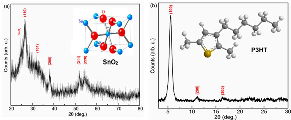
Figure 2. X-ray diffraction patterns of (a) sputtered SnO 2 deposited on quartz substrate and (b) P3HT spin-coated on glass substrate.
