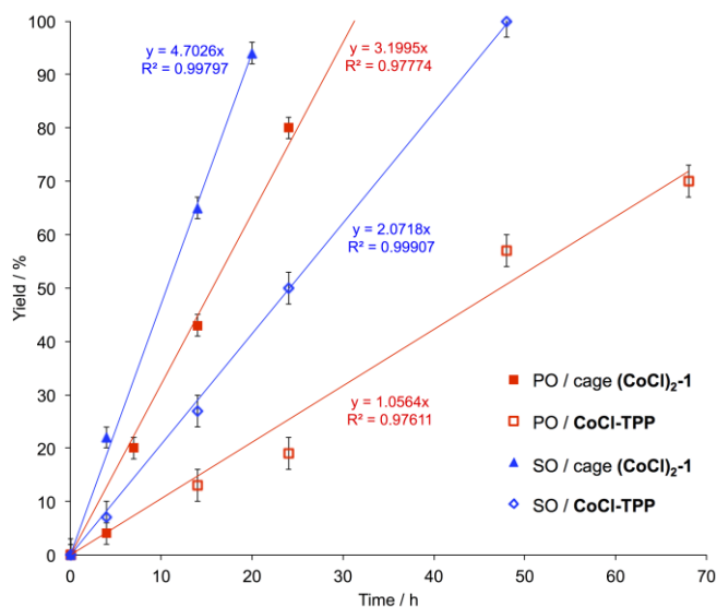
Figure 4. Kinetics of the conversion of styrene oxide (SO) or propylene oxide (PO) to the corresponding cyclic carbonates catalysed by cage (CoCl) 2 -1 or reference porphyrin CoCl-TPP . Reaction conditions: SO or PO (3.57 mmol, 1.1 M in DCM), 0.2 mol% in porphyrin, pyridine 1.2 mol%, 120 °C, 20 bar.
