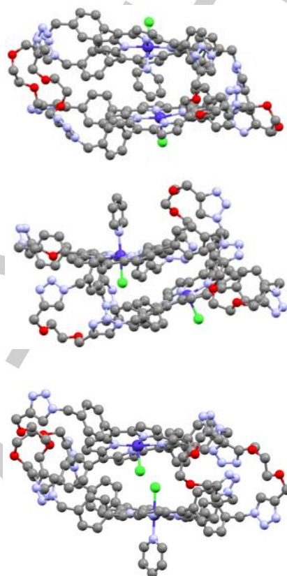
Figure 3. Optimized geometry of the out-out (top), in-out (middle) and in-in conformers (bottom) of the (CoCl) 2 -1 complexed with a pyridine. H atoms are hidden for clarity.
