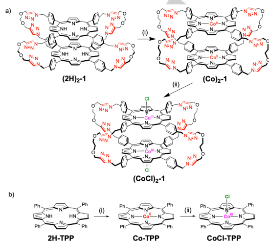
Scheme 1. a) Synthesis of ( (CoCl) 2 - 1 ): [21] (i) Co(OAc) 2 ·4H 2 O (20 equiv), DMF, Ar, 150 °C, 2 h; (ii) HCl 37%, air, DCM/MeOH (9:1), 24 h, 86%; b) Synthesis of CoCl-TPP : (i) Co(OAc) 2 ·4H 2 O (5 equiv), DMF, Ar, 150 °C, 1 h; (ii) HCl 37%, air, MeOH, 24 h, 93%.
