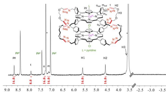
Figure 1. 1 H NMR (CDCl 3 /1% pyridine- d 5 , 300 MHz, 298 K) of cage ( (CoCl) 2 - 1 ). [23] *: Residual solvents. Pyr : pyridine.
