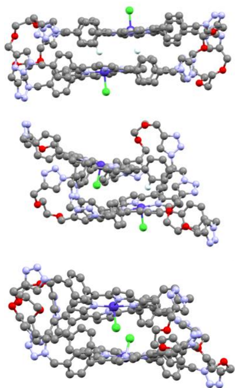
Figure 2. Optimized geometry of the lowest energy conformers out-out (top), in-out (middle) and in-in (bottom) of the (CoCl) 2 -1 complex. Only the H atom interacting with the cobalt(III) metal ions are shown, the others were removed for clarity.
