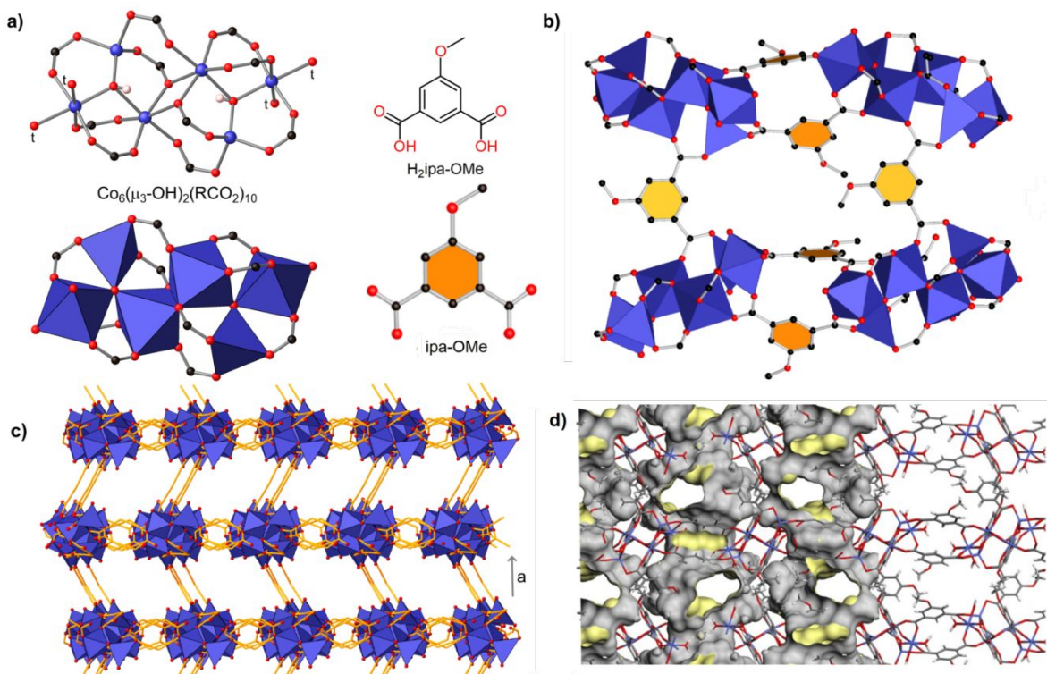
Figure 1. (a) The SCXRD structure of MUF-15-OMe comprises hexanuclear cobalt(II) clusters (cobalt = dark blue; oxygen = red; carbon = gray; hydrogen = pale pink (mostly omitted for clarity)) connected by 5-methoxyisophthalate (ipa-OMe) linkers. Sites occupied by terminal H 2 O ligands are marked with the letter t. (b, c) Cobalt(II) clusters and ipa-OMe ligands assemble into a network that defines a 3D array of channels in MUF-15-OMe. Each cluster is connected to ten others by bridging ipa-OMe ligands. (d) The network of pores in MUF-15-OMe illustrated by the Connolly surface in yellow (probe of diameter 1.0 Å). The outer surface of the pore space network is shown in grey
