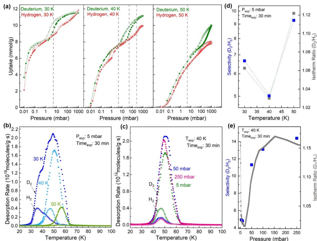
Figure 4. (a) Semi-logarithmic representation of MUF-15-OMe isotherms for H 2 and D 2 at 30, 40 and 50 K. The grey lines indicate the conditions at which TDS measurements with a 1:1 isotope mixture were performed. (b) Desorption of MUF-15-OMe for 30, 40 and 50 K exposure temperature: TDS desorption rate at 5 mbar exposure pressure and 30 min exposure time. (c) Desorption of MUF-15-OMe for 5, 50 and 250 mbar exposure pressure: TDS desorption rate at 40 K exposure temperature and 30 min exposure time. Selectivity determined by TDS and isotope ratio of MUF-15-OMe as a function of exposure temperature (d) and of exposure pressure (e). The isotherm ratio was determined for 52 pressure points, TDS measurements were carried out at four different pressures.
