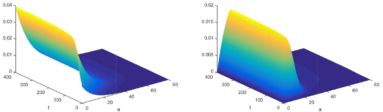
FIGURE 11. The evolution of solutions i (left) and q (right) with respect to time t and age a .
