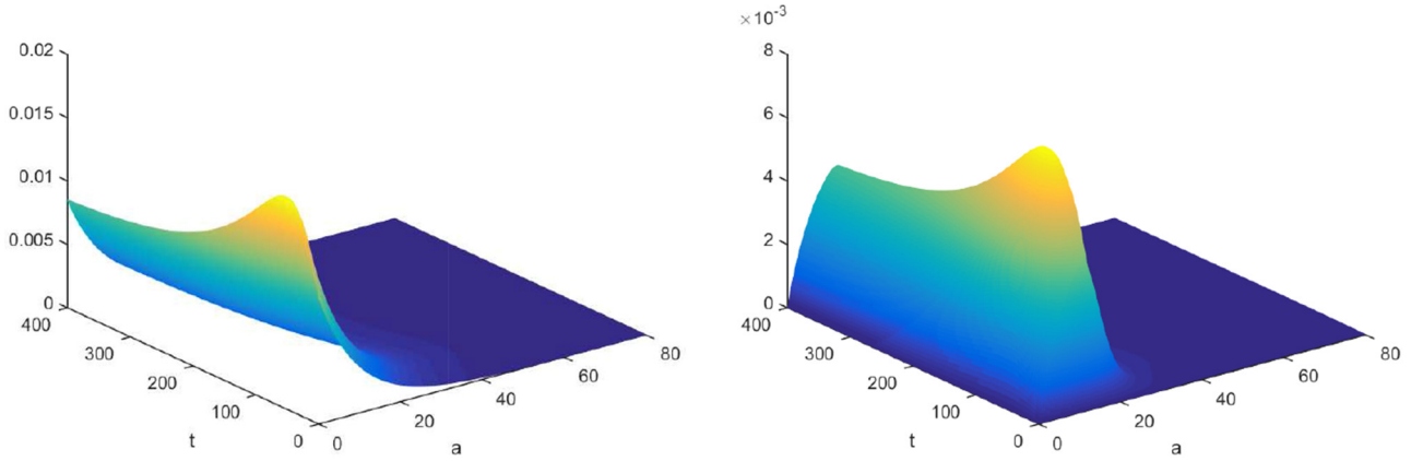
FIGURE 5. The evolution of solutions i (left) and q (right) with respect to time t and age a .
