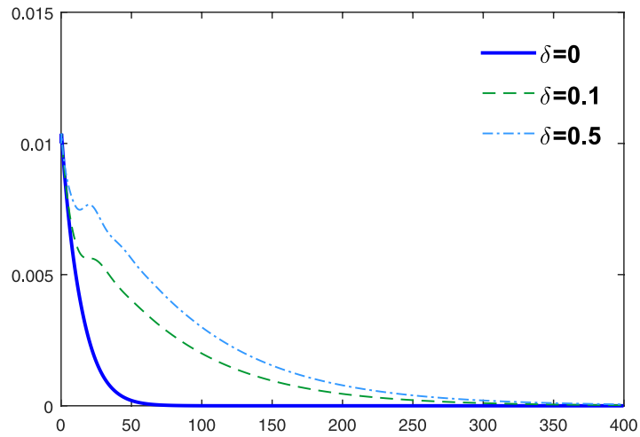
FIGURE 9. The evolution of i(t, 0) with respect to time t .
