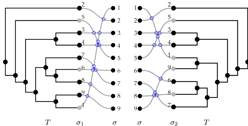
Figure 5 Two planar embeddings of a rooted tree T : the one on the left is optimal for the OTDE problem (deleting the 3 gray leaves makes the order \sigma suitable on T restricted to the remaining leaves, but the order \sigma_1 suitable on T has 11 inversions, shown with empty circles, with \sigma ); the other one is optimal for the OTCM problem with the order \sigma_2 suitable on T having 10 inversions with \sigma but not for the OTDE problem (4 leaves, for example the 4 gray ones, need to be deleted to make the order \sigma suitable on T restricted to the remaining leaves).
