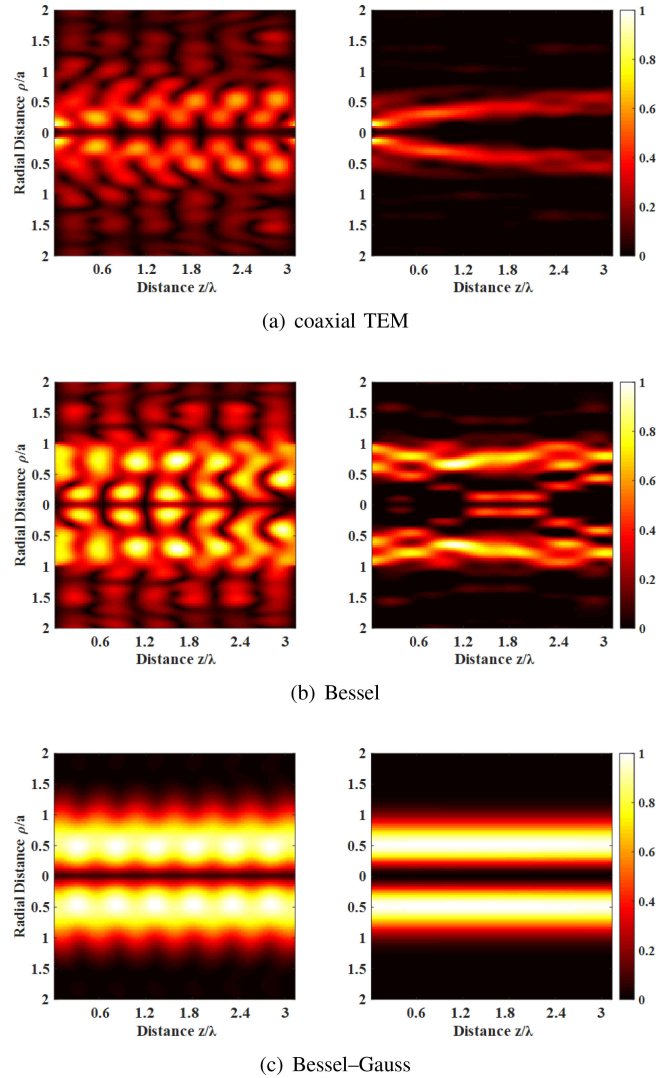
FIGURE 6. Normalized amplitudes of the E-field and the z-component of the Poynting vector in the x0z plane between two apertures when L = 3.15\lambda . The electric field is plotted on the left, and the Poynting vector is plotted on the right. (a) TEM, (b) BB, and (c) BGB distribution.
