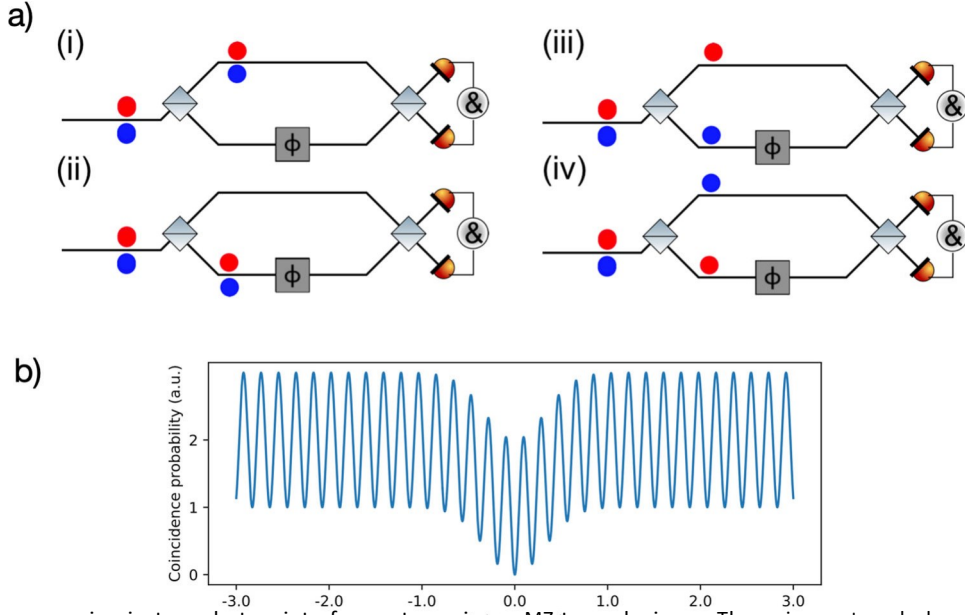
Fig. 1 Different case scenarios in two-photon interferometry using an MZI-type device. a The pair can travel along four different paths. Interference in the coincidence counts can occur provided two paths are indistinguishable. Note that the different colors for the two photons are for representation purpose only. Ideally the paired photons are indistinguishable. b Interference pattern at the output of a balanced interferometer.
