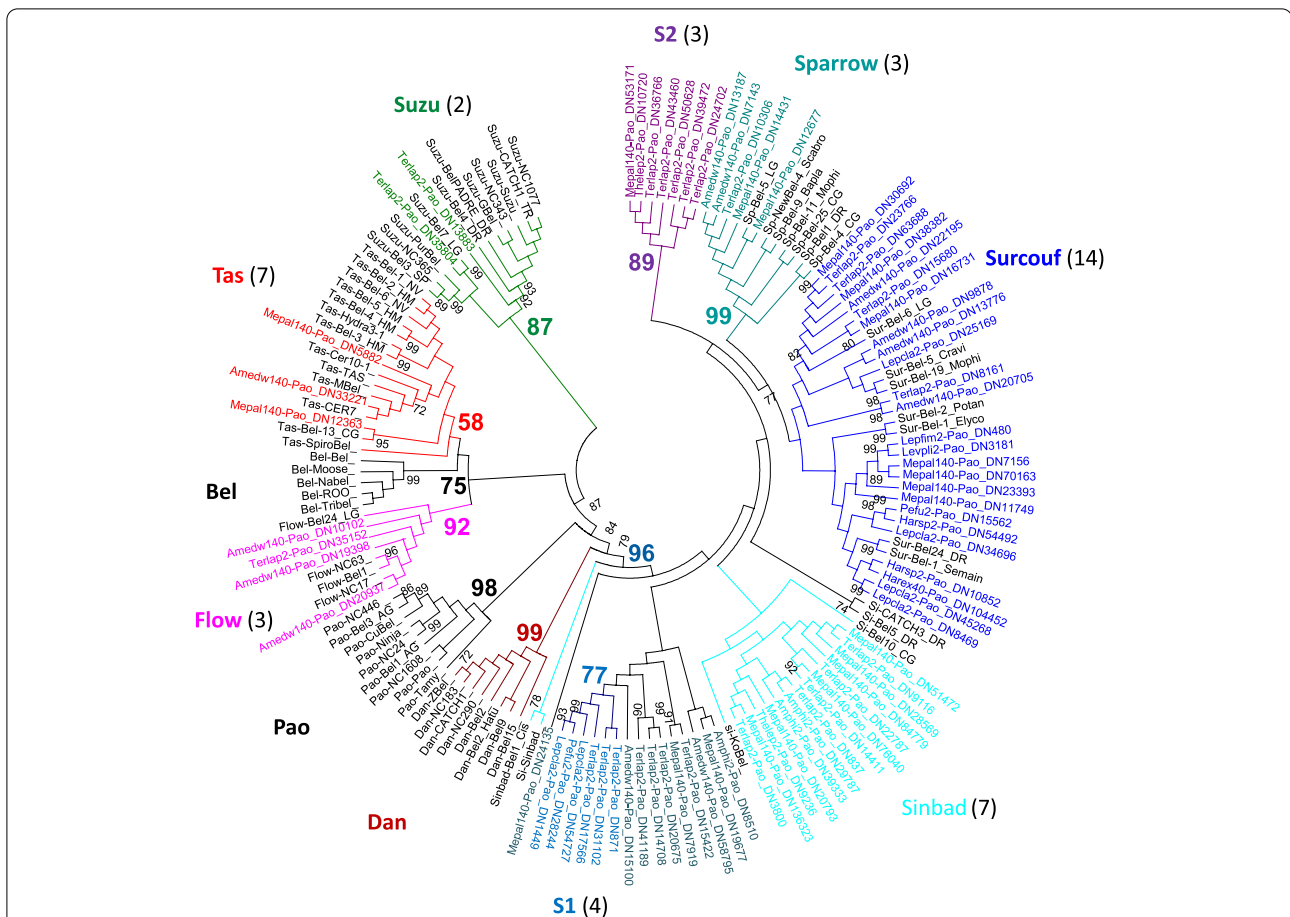
Fig. 8 Phylogenetic relationships of BEL/Pao retrotransposons. The tree is based on Neighbor-Joining analysis of RT/RNaseH domain amino acid sequences. The BEL/Pao families from annelids are indicated in color, as are the major clades to which they belong. The number of annelid species covered by each clade (evaluated on both RT/RNaseH and Integrase domains) is given between brackets. Node statistical support values (> 70%) come from non-parametric bootstrapping using 100 replicates
