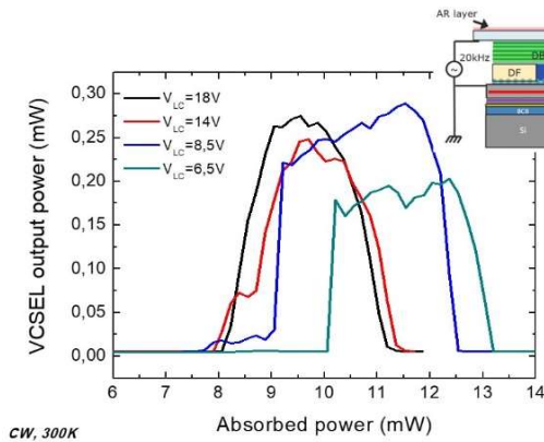
Fig. 1. VCSEL output power as function of pump absorbed power for different voltages applied on the LC \mu cell (20 kHz). Insert is a schematic of the LC \mu cell VCSEL
