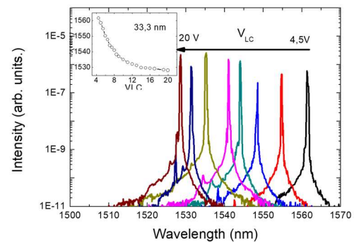
Fig. 2. VCSEL spectra measured at pump power of 10 mW, for different LC applied voltages (20 kHz). Insert shows the VCSEL lasing wavelength as function of the LC applied voltage.
