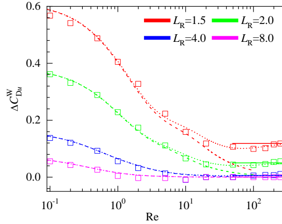
FIG. 11. Wall-induced drag correction \Delta C_{Du}^W for a non-rotating sphere translating parallel to a wall in a fluid at rest in the range 0.1 \leq \text{Re} \leq 250 . Symbols: numerical data; solid lines: high-Re correction (28); dashed lines: low-to-moderate-Re correction (27); dotted lines: composite fit (29).
