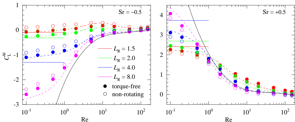
FIG. 23. Influence of the sphere rotation induced by the torque-free condition on the lift force for |\text{Sr}| = 0.5 and 0.1 \leq \text{Re} \leq 150 . Closed and open symbols refer to the lift coefficient for torque-free and non-rotating spheres, respectively. Horizontal solid lines: asymptotic prediction (16) corresponding to conditions L_u \ll 1 , L_w \ll 1 , L_\Omega \ll 1 ; dashed lines: empirical prediction (41); black solid line: total lift coefficient for a torque-free sphere in an unbounded shear flow (fitted from the results obtained with the present code).
