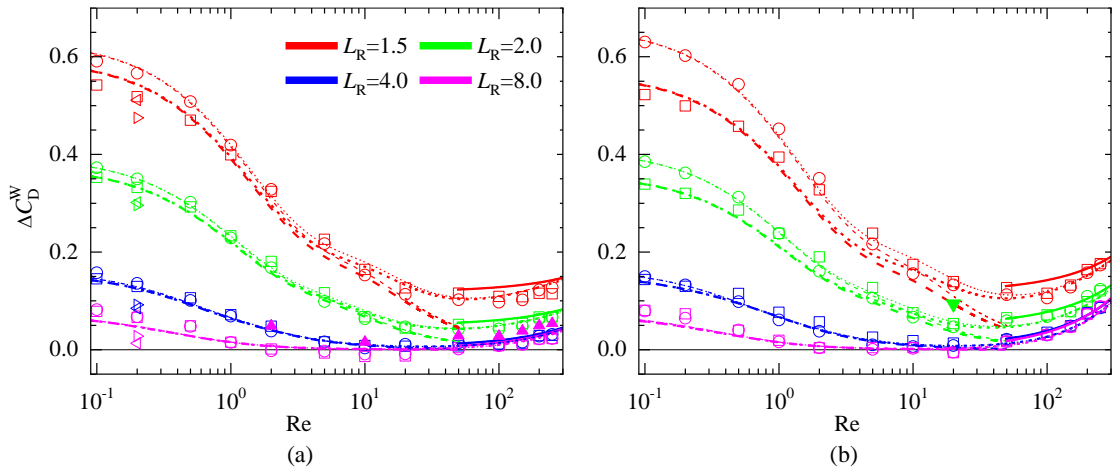
FIG. 16. Relative near-wall drag increase \Delta C_D^W(\text{Re}, Sr, L_R) for a non-rotating sphere translating parallel to a wall in a linear shear flow, throughout the Re-range investigated numerically. (a) Sr = \pm 0.2 ; (b) Sr = \pm 0.5 . \square and \circ : present numerical data for Sr > 0 and Sr < 0 , respectively; \triangleleft and \triangleright : numerical data from [29] for Sr = -0.2 and Sr = +0.2 , respectively; \blacktriangle : numerical data from [17] for Sr = 0.25 ; \blacktriangledown : numerical data from [30] for Sr = +0.5 . Thick solid lines: high-Re model based on the sum of (28) and (33); thick (thin) dashed lines: low-to-moderate-Re expression (31) for positive (negative) Sr ; thick (thin) dotted lines: composite fit (34) for positive (negative) Sr .
