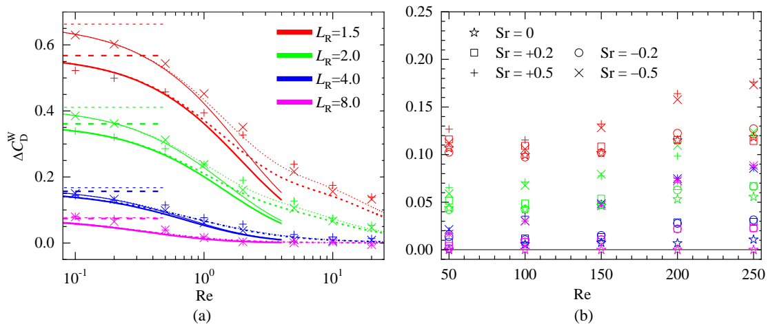
FIG. 13. Relative near-wall drag increase \Delta C_D^W for a non-rotating sphere translating parallel to a wall in a linear shear flow. (a): low-to-moderate Reynolds number regime for Sr = \pm 0.5 ; (b): moderate-to-high Reynolds number regime for Sr = \pm 0.2 and \pm 0.5 . Symbols in (a): numerical results for Sr = 0.5 (+) and Sr = -0.5 (×). Dashed lines: asymptotic prediction (18) corresponding to conditions L_u \ll 1 , L_\omega \ll 1 ; solid lines: low-but-finite-Re semiempirical expression (23); dotted lines: low-to-moderate-Re semiempirical expression (31). Thick (thin) lines correspond to positive (negative) Sr .
