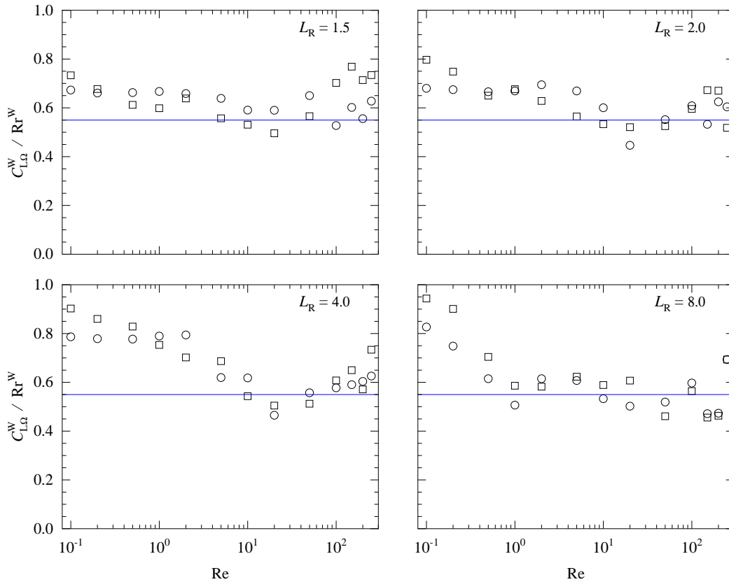
FIG. 24. Change in the lift coefficient due to the sphere rotation induced by the torque-free rotation. Values of C_{L\Omega}^W are divided by the rotation rate Rr^W to provide a better collapse. \square and \circ symbols refer to numerical data for Sr > 0 and Sr < 0 , respectively. Solid lines: approximation C_{L\Omega}^U/Rr \approx 0.55 established in [11] in an unbounded shear flow.
