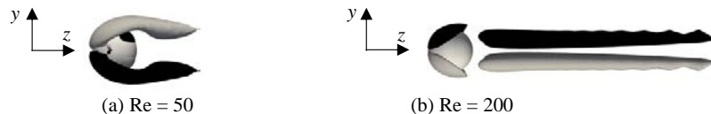
FIG. 6. Iso-surfaces of the streamwise vorticity in the wake of a sphere moving in an unbounded linear shear flow with Sr = 0.5 (the black thread corresponds to the positive value). (a) Re = 50 , d/(2|U_{rel}|\omega \cdot e_z) = \pm 0.1 ; (b) Re = 200 , d/(2|U_{rel}|\omega \cdot e_z) = \pm 0.25 . The relative upstream flow is from left to right and the free vorticity -\gamma lies along the y -direction.
