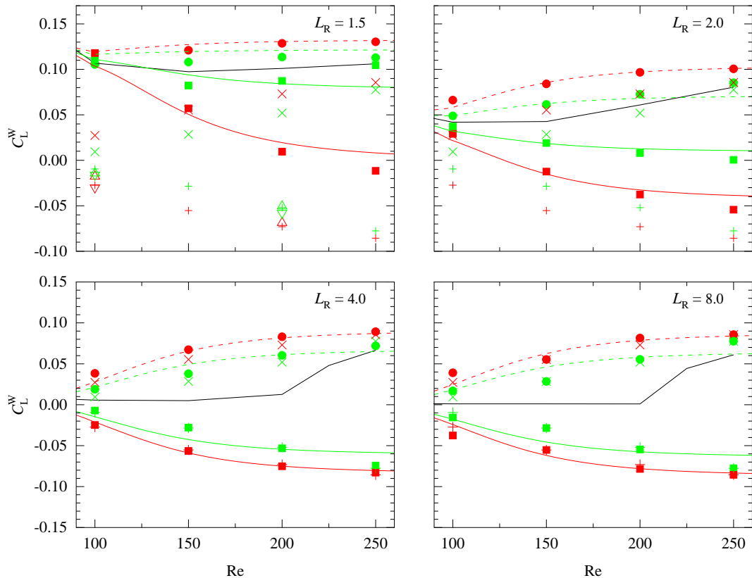
FIG. 19. Variations of the lift coefficient C_L^W(\text{Re}, \text{Sr}, L_R) in the range 100 \leq \text{Re} \leq 250 for a non-rotating sphere translating parallel to a wall in a linear shear flow. \blacksquare : \text{Sr} = +0.2 , \bullet : \text{Sr} = -0.2 , \blacksquare : \text{Sr} = +0.5 , \bullet : \text{Sr} = -0.5 . Unbounded shear flow: + and + (all panels): \text{Sr} = +0.5 and +0.2 , respectively; same with \times and \times for \text{Sr} = -0.5 and -0.2 , respectively; \triangle and \triangle (top left panel): data from [9] for \text{Sr} = +0.5 (interpolated) and \text{Sr} = +0.2 , respectively; \nabla and \nabla (top left panel): data from [11] for \text{Sr} = +0.4 and \text{Sr} = +0.2 , respectively. Black solid line: \text{Sr} = 0 ; green solid (dashed) line: prediction (37) for \text{Sr} = +0.2 ( -0.2 ); same with the red solid (dashed) line for \text{Sr} = +0.5 ( -0.5 ).
