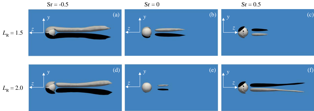
FIG. 4. Iso-surfaces d/(2|U_{\text{rel}})|\omega \cdot e_z = \pm 0.25 of the streamwise vorticity in the wake of a sphere moving parallel to a wall at \text{Re} = 200 (the black thread corresponds to positive values). Left column: \text{Sr} = -0.5 ( U_{\text{rel}} < 0 ); central column: \text{Sr} = 0 ( U_{\text{rel}} < 0 ); right column: \text{Sr} = 0.5 ( U_{\text{rel}} > 0 ). The flow with respect to the sphere is from left to right, i.e. in the z -direction for \text{Sr} = 0.5 and in the -z -direction for \text{Sr} = 0 and -0.5 . Since (x, y, z) is right-handed, the wall stands at the back of the sphere for \text{Sr} = 0.5 and at its back for \text{Sr} = 0 and -0.5 .
