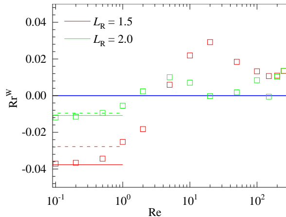
FIG. 20. Variations with Re and L_R of the rotation rate Rr^W of a torque-free sphere translating parallel to a wall in a fluid at rest. Symbols: numerical results; dashed lines: asymptotic prediction (17) corresponding to the condition L_u \ll 1 ; solid lines: empirical extension (39) of (17) based on the exact zero- Re prediction of [38, 49].
