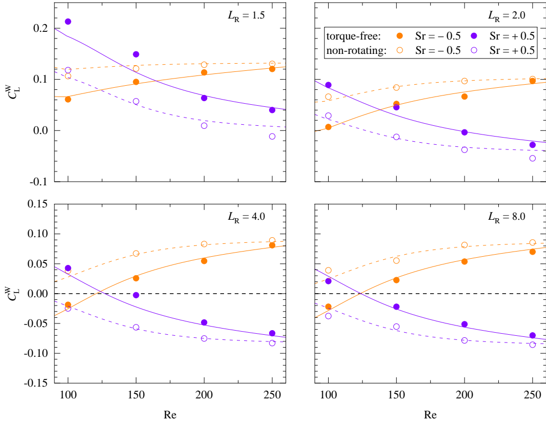
FIG. 25. Influence of the torque-free rotation on the lift force in the high-Reynolds-number regime for |\text{Sr}| = 0.5 . Closed and open symbols refer to data obtained with torque-free and non-rotating spheres, respectively. Solid and dashed lines correspond to the prediction of (42) for the torque-free and non-rotating cases, respectively. The horizontal black dashed line materializes the dividing line C_L^W = 0 .
