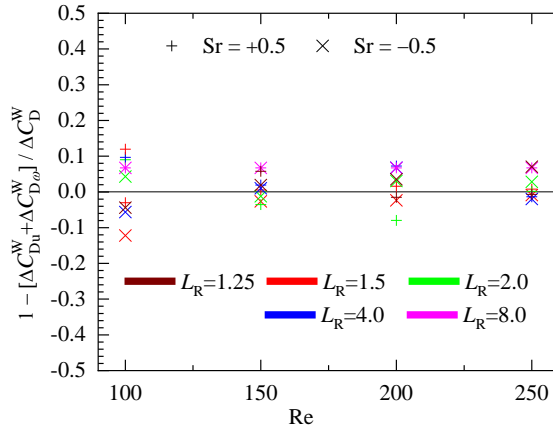
FIG. 15. Comparison for Sr = \pm 0.5 of the measured near-wall drag increase \Delta C_D^W in the high-Reynolds-number regime with the prediction \Delta C_{Du}^W[\text{Re} = O(100)] + \Delta C_{D\omega}^W[\text{Re} = O(100)] provided by the empirical models (28) and (33).
