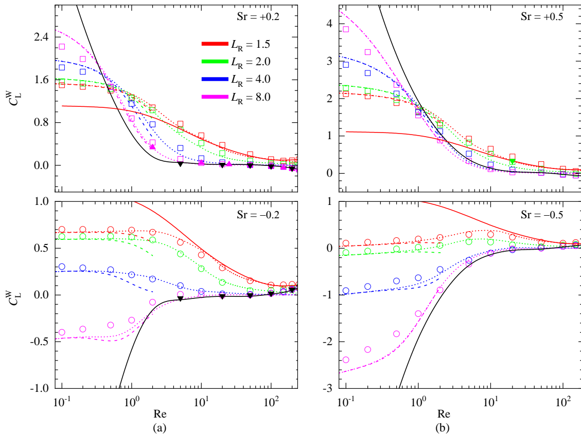
FIG. 18. Lift coefficient C_L^W(\text{Re}, \text{Sr}, L_R) for a non-rotating sphere translating parallel to a wall in a linear shear flow at \text{Re} \leq 150 . (a) \text{Sr} = \pm 0.2 ; (b) \text{Sr} = \pm 0.5 . \square and \circ : numerical data for \text{Sr} > 0 and \text{Sr} < 0 , respectively. \blacktriangle : numerical data from [17] for \text{Sr} = 0.25 ; \blacktriangledown : numerical data from [30]; \blacktriangledown data from [11] in the unbounded configuration. Dashed lines: finite-Re prediction (21); dotted lines: prediction (35); black solid lines: lift coefficient C_{L\omega}^U in an unbounded shear flow (fitted from the results obtained with the present code); red solid lines: lift coefficient C_{Lu}^W at L_R = 1.5 in a wall-bounded fluid at rest.
