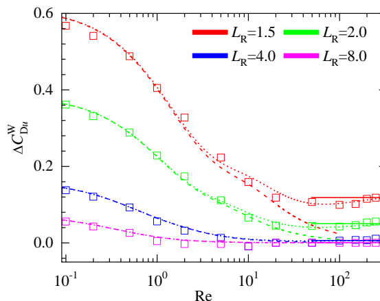
FIG. 11. Wall-induced drag correction \Delta C_{Du}^W for a non-rotating sphere translating parallel to a wall in a fluid at rest in the range 0.1 \leq Re \leq 250 . Symbols: numerical data; solid lines: high-Re correction (28); dashed lines: low-to-moderate-Re correction (27); dotted lines: composite fit (29).
