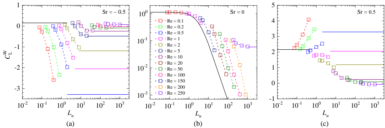
FIG. 26. Variations of the lift force vs. the separation-based Reynolds number L_u for torque-free spheres translating at various Reynolds numbers in a wall-bounded flow. (a): Sr = -0.5 (the sphere leads the fluid); (b) Sr = 0 (the fluid is at rest at infinity); (c): Sr = +0.5 (the sphere lags behind the fluid). Symbols: numerical results. Solid lines on the right part of each panel: asymptotic value of C_L in the unbounded configuration ( L_u \rightarrow \infty ); solid line on the left part of panels (a) and (c): asymptotic prediction (16) evaluated in the limit L_R \rightarrow 1 (sphere touching the wall); black solid line in (b): prediction (20) from [14] valid for Re \ll 1 and L_u \gg 1 .
