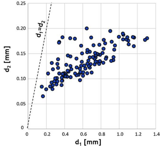
Fig. 5. Relationship between the diameter of the injected bubble and the diameter of the fragmented bubble in 30% glycerol aqueous solution, which has a viscosity 2.5 times that of water, measured at a throat flow velocity of u_{th} = 11.5 m/s ( Q = 2.10 l/min).
