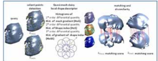
Quasi-mesh-daisy local shape descriptor based free-form surface matching framework.
