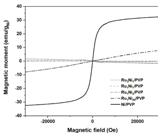
Figure 4. Magnetic hysteresis cycles of bimetallic and monometallic nanoparticles measured at room temperature.
