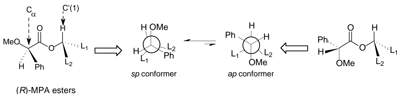
Scheme 5. NMR- significant conformers of ( R )-MPA esters.
