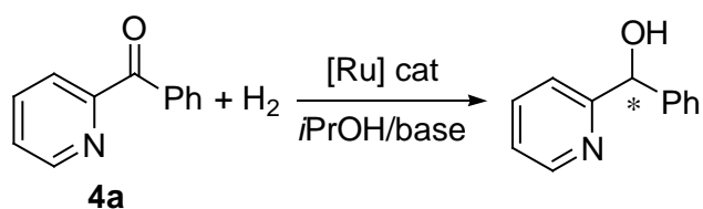
Scheme 3. Hydrogenation of phenyl pyridinyl methanone 4a .
