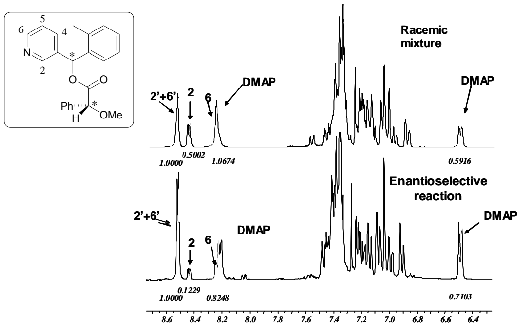
Figure 5. ^1\text{H} NMR spectra of 9b esters resulting from ( R )-MPA and crude mixture of alcohols obtained from the hydrogenation of 5b .
