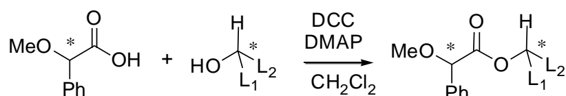
Scheme 4. Synthesis of methoxy-phenyl-acetic acid esters.
