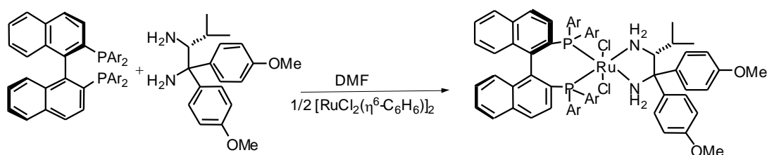
Scheme 2. Synthesis of ruthenium precatalysts.
