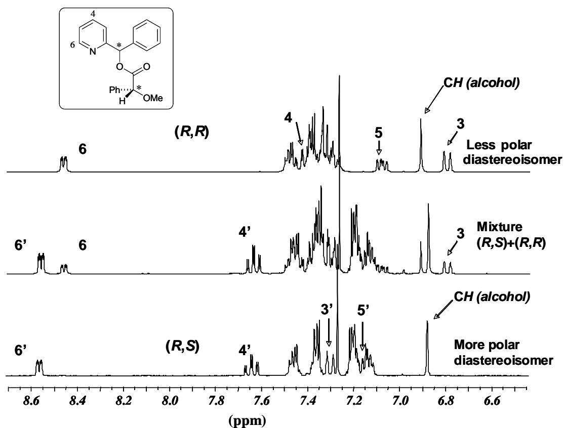
Figure 1. Partial ^1\text{H} NMR spectra of ( R )- and ( S )- 8a esters of ( R )-MPA (a) less polar diastereomer (b) mixture of diastereomers (c) more polar diastereomer.
