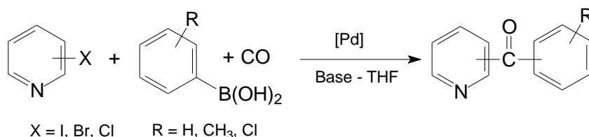
Scheme 1. Synthesis of pyridinyl aryl ketones via carbonylative Suzuki coupling.
