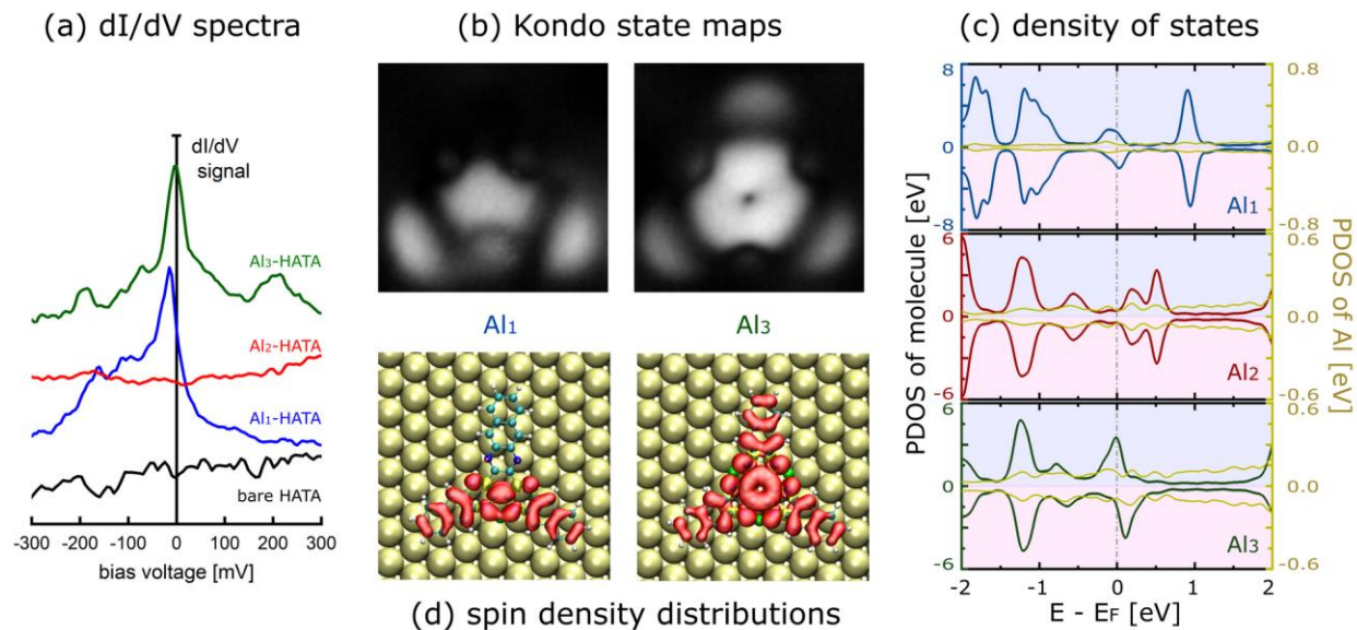
Figure 2: (a) The dI/dV tunneling spectra around the Au(111) surface Fermi level recorded by positioning the STM tip apex at the center of molecule for each complex. For each bias voltage, those spectra were recorded using a lock-in amplifier with an 8 mV of voltage modulation. (b) The dI/dV differential conductance maps of the Al 1 - and Al 3 -HATA complexes at recorded at -15 mV. Those conductance maps are presented contrast inverted because the -15 mV scanning bias voltage was set up slightly higher than the blue and dark-green Kondo resonance maxima in (a) to secure enough the distance between the STM tip end apex and the HATA molecule. It fully reflects the state lying toward the low energy region. 25 (c) DFT calculated projected densities of states (PDOS) for the three HATA complexes showing the magnetic character of the Al 1 - and Al 3 -HATA complexes. (d) The DFT calculated spin density maps of the Al 1 -HATA and Al 3 -HATA complexes. Al 2 -HATA is not presented because of no spin polarization in this case.
