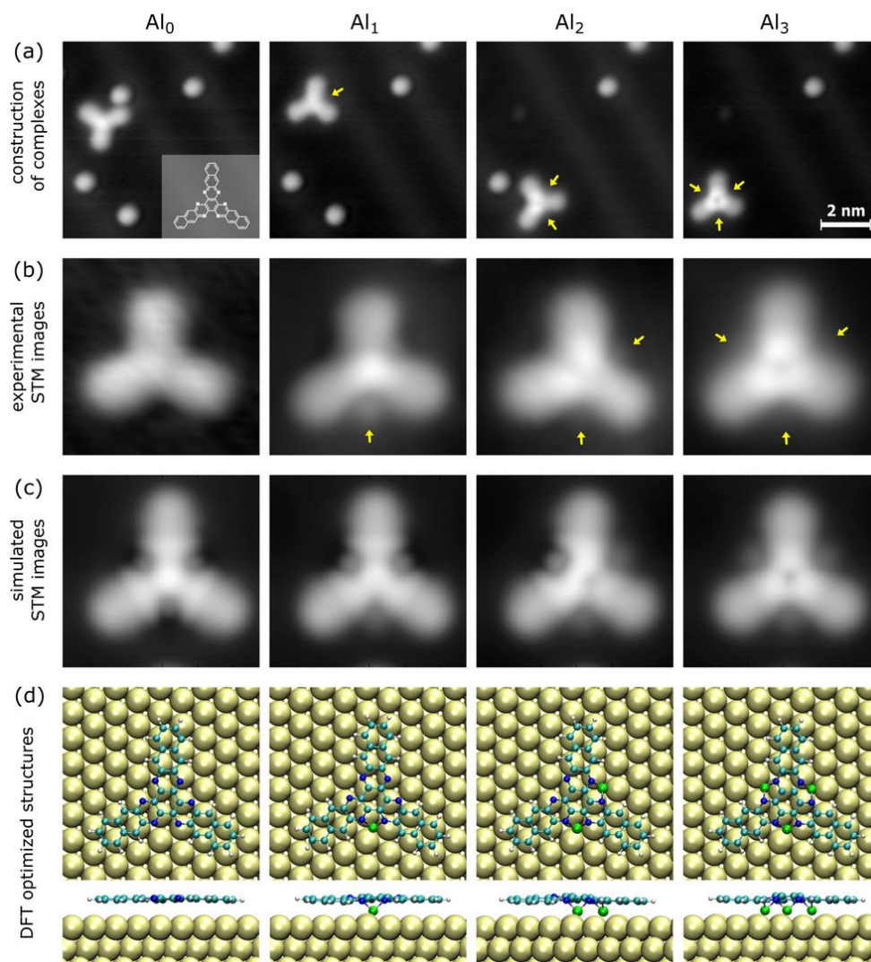
Figure 1. (a) From left to right, the one by one construction of the aluminum organometallic complexes up to three Al atoms on the HATA molecule. The STM images were recorded at 500 mV bias voltage and 200 pA constant tunneling current intensity. The chemical structure of the hexaazatrianthracene (HATA) molecule is inserted in the leftmost image in (a). (b) Experimental STM zoomed-in images of \text{Al}_x\text{-HATA} molecules ( x = 0, 1, 2, and 3 from left to right) where the single Al coordinated ad-atoms can be observed (Yellow arrows). (c) The corresponding simulated STM images using the optimized HATA surface structures presented in (d) resulting from DFT calculations.
