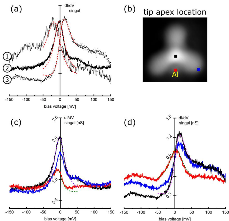
Figure 3: (a) the change of the dI/dV tunneling spectral shape (Kondo-Fano resonance) at the center of Al_1 -complex before and after the STM manipulation of this complex. ① Asymmetric shape with a peak at the negative energy side (Fano asymmetry parameter q = -5 ) just after the construction of the complex. ② After STM manipulating this complex laterally on the surface, the resonance becomes almost symmetrical ( q = 40 ). ③ Further lateral manipulations resulted in an asymmetrical shape with a resonance peak on the positive energy side ( q = 2 ). After the change by those lateral manipulation of resonance peak shape, the dI/dV spectra were recorded at different tip locations indicated in (b). The Kondo character of the resonances measured at the center of molecule (black colored) and at the end of the anthracene branch (blue colored) is the same in (c) and (d). However, the peak shape recorded on the Al sites (red colored) is different because of the change of the Al atom position. All smooth dotted lines are the Kondo fitting based on the Fano theory. 19
