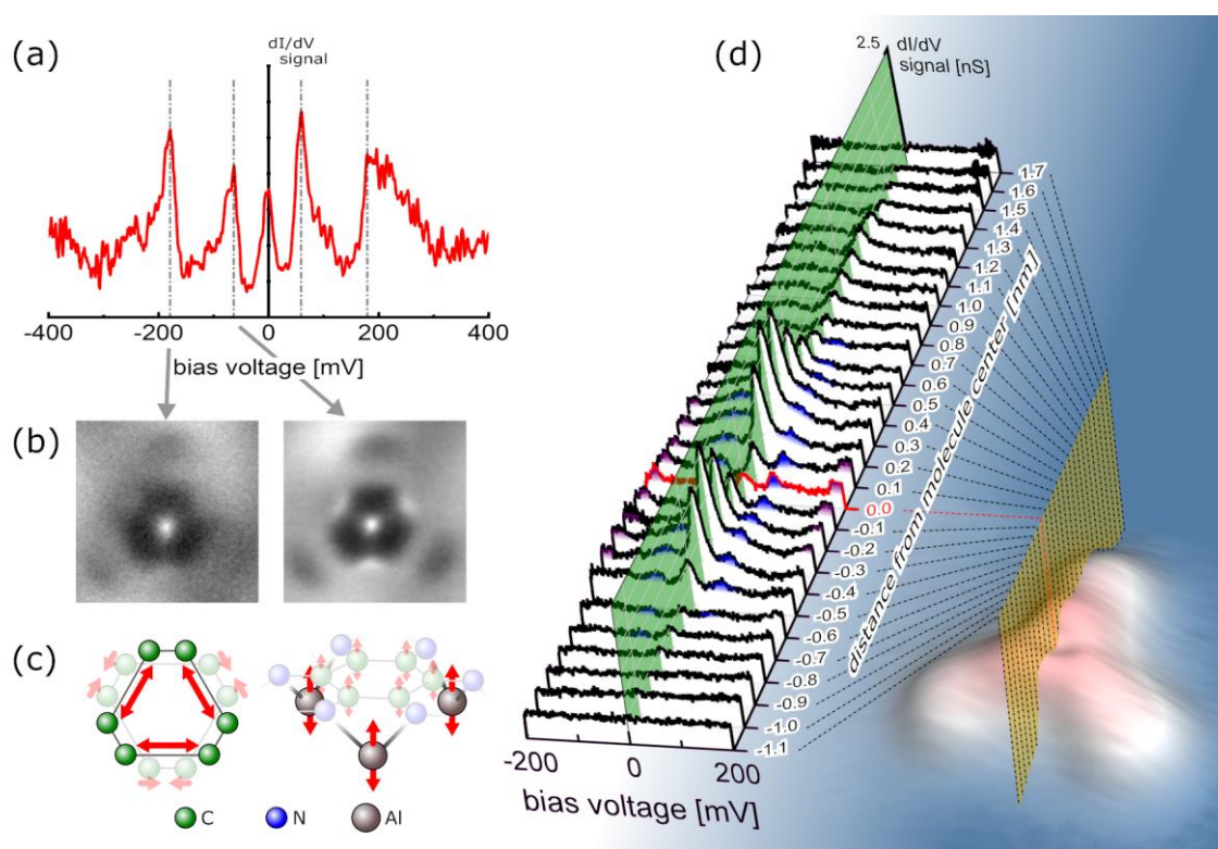
Figure 4: (a) The dI/dV spectrum exactly recorded at the center of the Al 3 -HATA molecular complex. (b) The differential conductance maps recorded at the energy of the two indicated different phonon channels. (c) The corresponding calculated vibrational modes at those energies. Each molecular vibration mode is collective motion here illustrated only with the corresponding core atoms. (d) a large series of spectra along the central line of the Al 3 -HATA complex. The low energy phonon peak can be followed along from -0.7 nm to 0.7 nm relative to the center of the molecule (blue painted). The high energy ones can be followed from -0.4 nm to 0.4 nm (purple).
