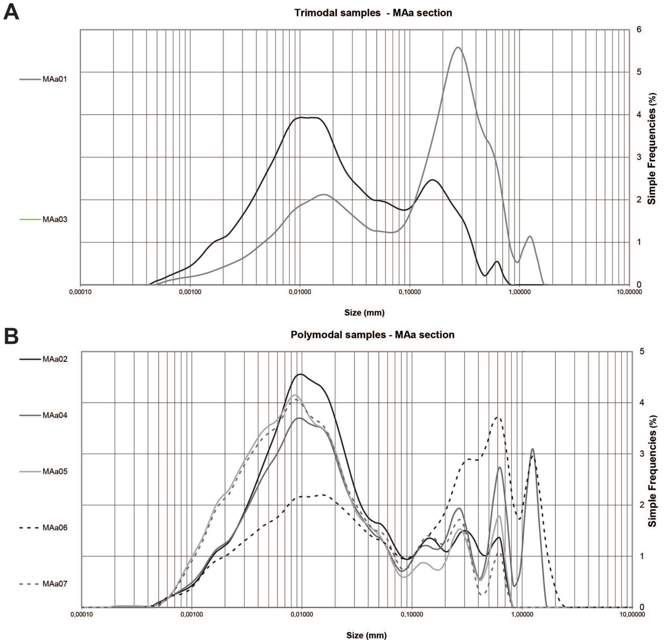
Fig. 15. Grain size curves, MAa section. A: Trimodal samples; B: Polymodal samples.
