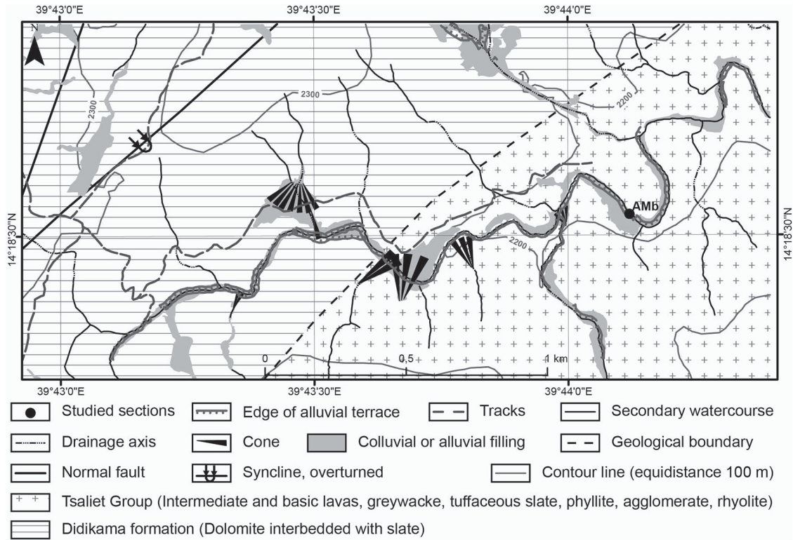
Fig. 8. Geomorphological sketch of Ambare Valley and its surroundings. Geological information after Kazmin (1976).
