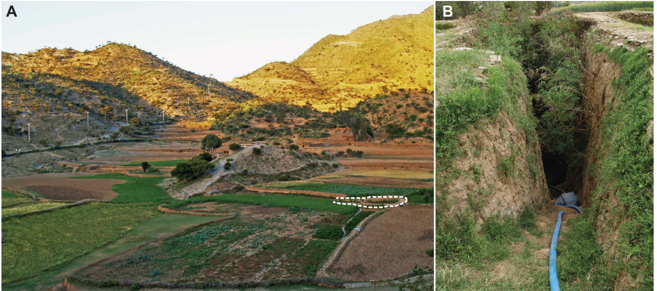
Fig. 6. A: Location of the MAa well in May Ayni Valley; B: MAa section in the well.
