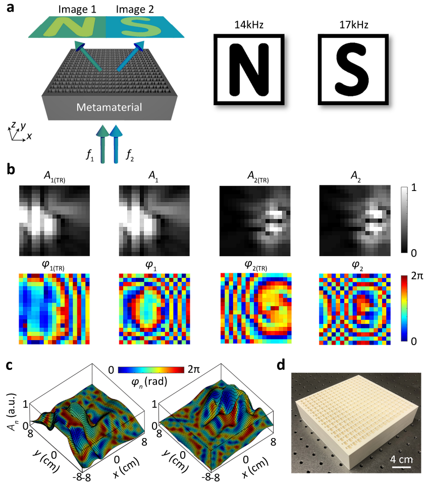
Figure 3. The holographic designs for letters “N” and “S” at 14 kHz and 17 kHz. (a) The predesigned holographic image at 14 kHz is letter “N”. The image plane is 5 cm away ( z = 5 cm) from the hologram plane. (b) The amplitude and phase distributions at hologram plane calculated by time reversal are (A_{n(TR)}, \varphi_{n(TR)}) . The final amplitude and phase distributions of the sample are calculated as (A_n, \varphi_n) . (c) The final distributions of (A_1, \varphi_1) and (A_2, \varphi_2) . (d) The photograph of the sample with a size of 18 cm \times 18 cm \times 4.5 cm with 17 \times 17 unit cells. Scale bar, 4 cm.
