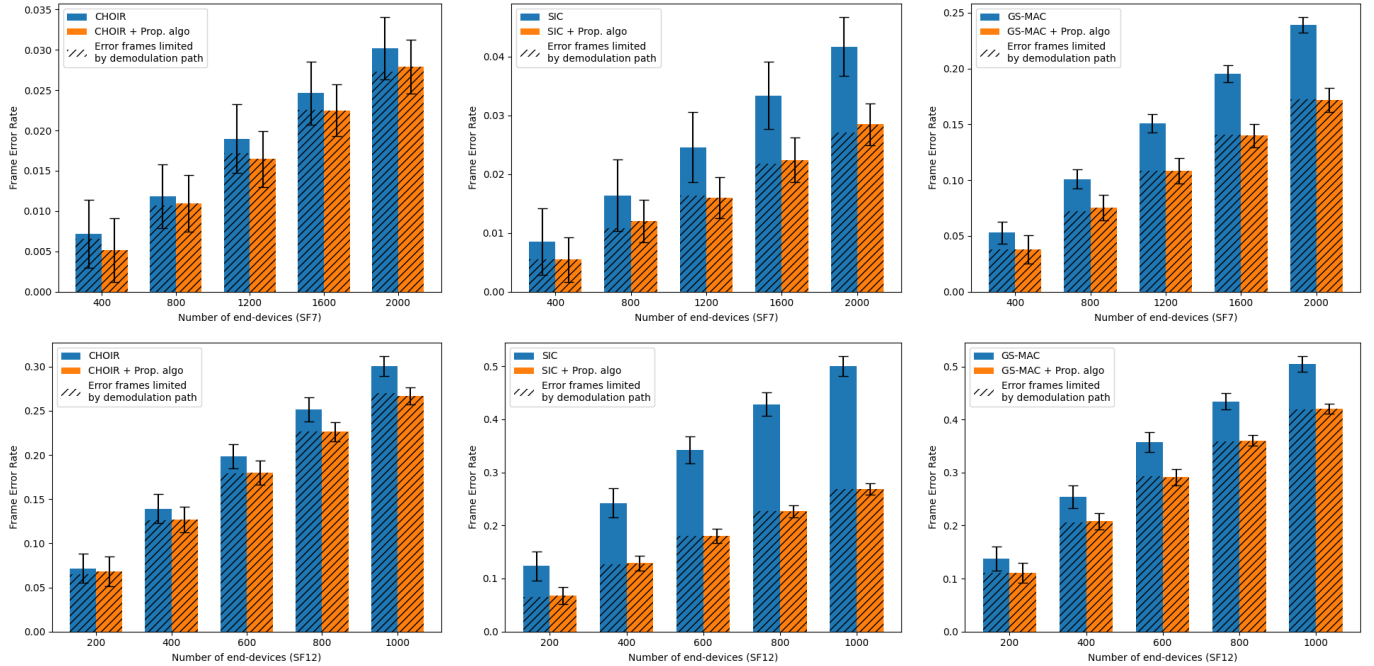
Fig. 5: Simulation results show that our proposed algorithm improves the decoding capacities for unconfirmed traffic with SF 7 and SF 12.
