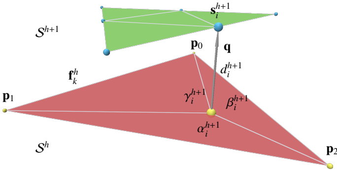
Fig. 4. Exploded view of the hierarchical structure: Vertex s_i^{h+1} of upper layer \mathcal{S}^{h+1} is linked to face f_k^h of lower layer \mathcal{S}^h . Vertex s_i^{h+1} position within f_k^h is encoded the barycentric coordinates (\alpha_i^{h+1}, \beta_i^{h+1}, \gamma_i^{h+1}) of its projection and its signed distance d_i^{h+1} from f_k^h .
