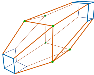
Fig. 3 A polytope considered by the inner step for (d, k, g) = (3, 4, 2) and \{u, v\} = \{(0, 0, 0), (4, 4, 4)\}
