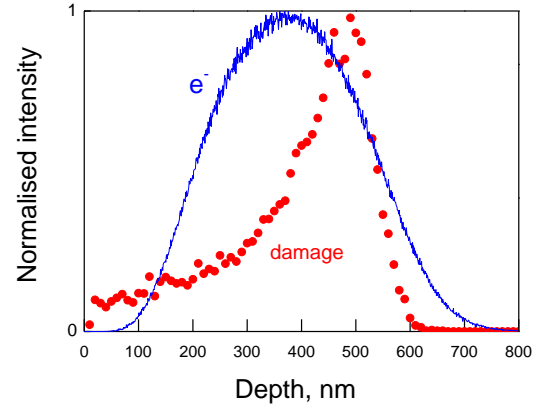
Fig. 5. Damage level induced by the He^+ ions (maximum value \sim 4-5 dpa) and normalised number of CL electrons (10 keV) in \gamma - Si_3N_4 sample.
