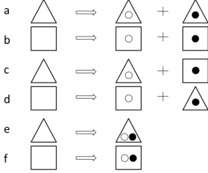
Fig. 9. Possible permutations of a cation between tetrahedral (Δ) and octahedral (□) voids resulting in formation of defects V_{Si} (○) and Si_{Vs} (●).
