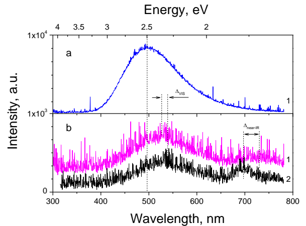
Fig. 6. PL spectra of \gamma - Si_3N_4 at T=9 K before (a) and after (b) irradiation with He^+ ions, with excitation at 5.39 eV (230 nm) (1) and 6.89 eV (180 nm) (2); \Delta E_1 = 150 meV and \Delta E_2 = 210 meV. The energy shifts of the visible and near-IR bands are opposite: \Delta_{near-IR} = -\Delta_{VIS} (where \Delta_{VIS} \equiv \Delta E_2 - \Delta E_1 \approx 60 meV).
