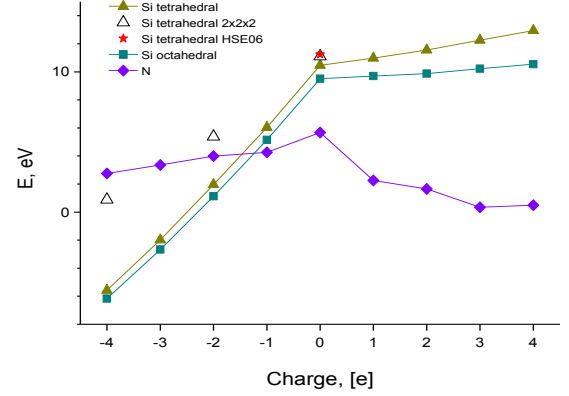
Fig. 10. Calculated trends in formation energy of charged cation (Si) and anion (N) vacancies in the spinel structure of \gamma - Si_3N_4 . (3)
