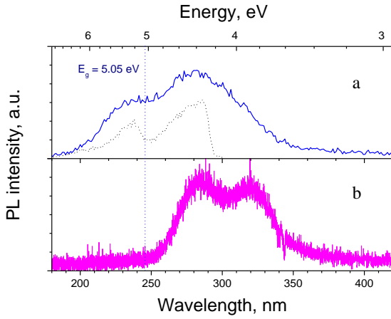
Fig. 7. PLE spectra at \lambda_{\text{PL}}=500 nm of \gamma - \text{Si}_3\text{N}_4 at T=9 K before (a) and after (b) irradiation with \text{He}^+ ions; dotted line shows PLE spectrum of the trapped exciton from Ref [15].
