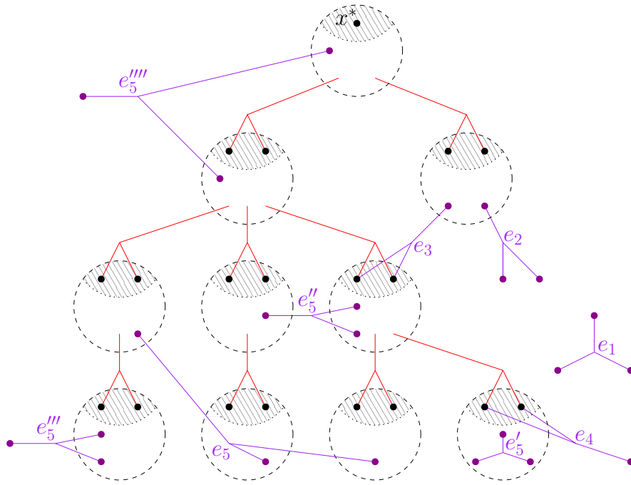
Figure 14: An arborescent archipelago \mathcal{A} (the inside of the islands is not detailed), and some edges in E(\mathcal{H}) \setminus E(\mathcal{A}) (in purple). The names of the edges follow the numbering from Definition 3.5: e_1 is of \mathcal{A} -type "exterior", e_2 is of \mathcal{A} -type "new crossing", etc.
