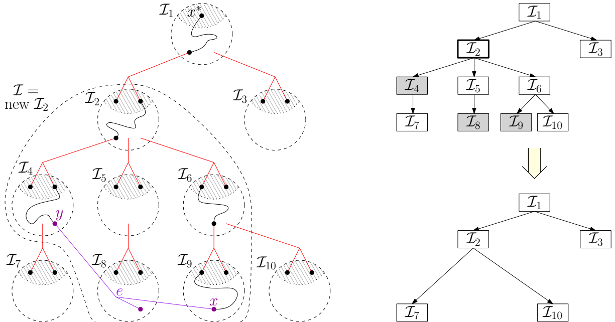
Figure 16: The archipelago \mathcal{A} \cup e where \mathcal{A} is as in Figure 14 and e = e_5 . On the right: the arborescences G(\mathcal{A}) (top) and G(\mathcal{A} \cup e) (bottom).
