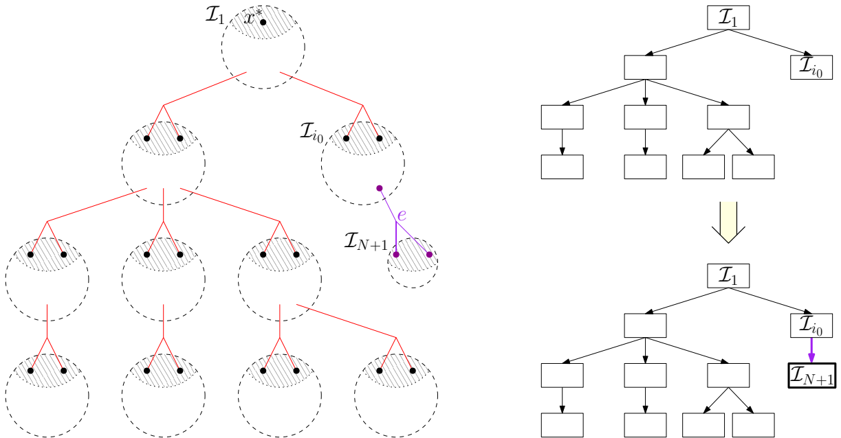
Figure 15: The archipelago \mathcal{A} \cup e where \mathcal{A} is as in Figure 14 and e = e_2 . On the right: the arborescences G(\mathcal{A}) (top) and G(\mathcal{A} \cup e) (bottom).
