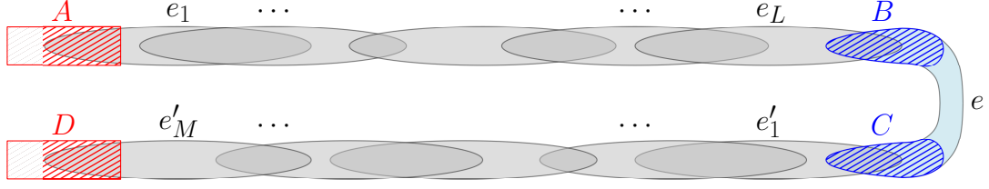
Figure 9: Illustration of Lemma 2.4.
