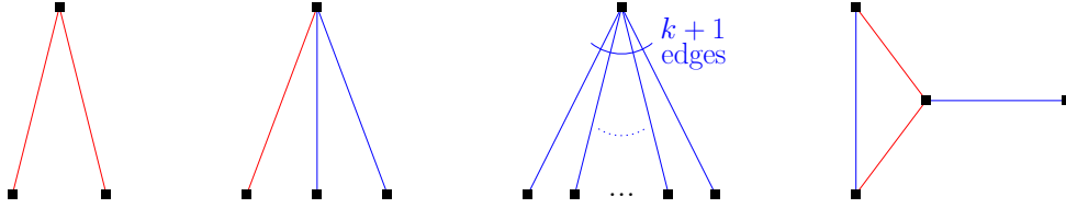
Figure 19: Some induced subgraphs that cannot appear in G \in \text{Im}(\varphi_{k,k-2}) .
