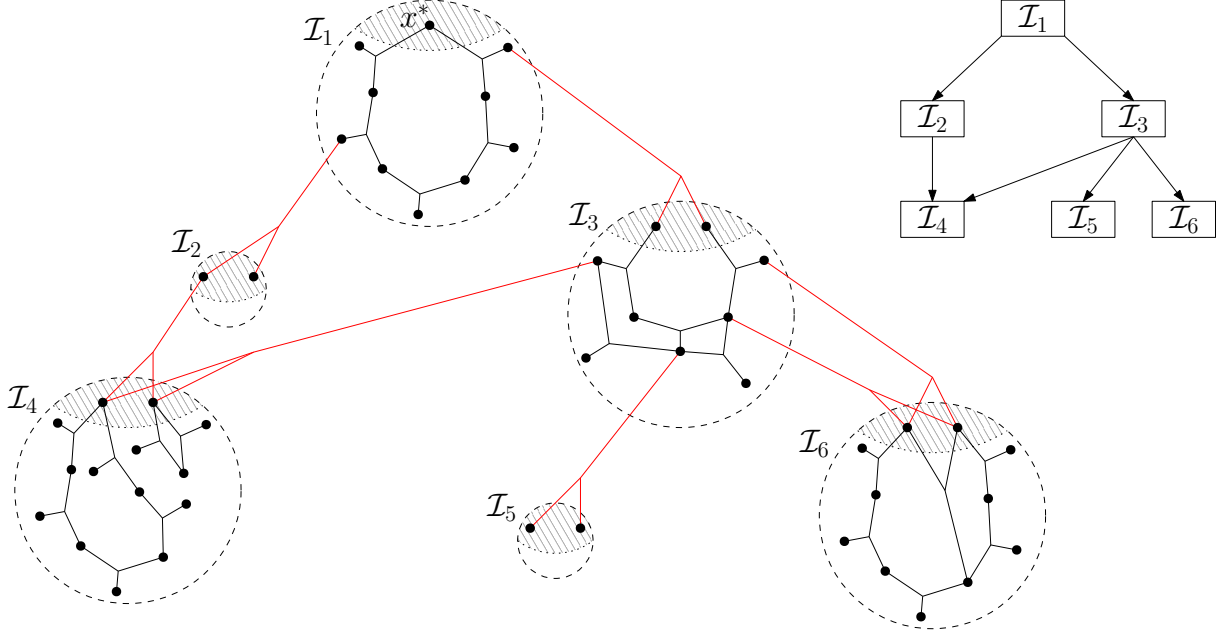
Figure 10: An archipelago which is not arborescent (with the digraph G on the right). Crossing edges will always be represented in red.
