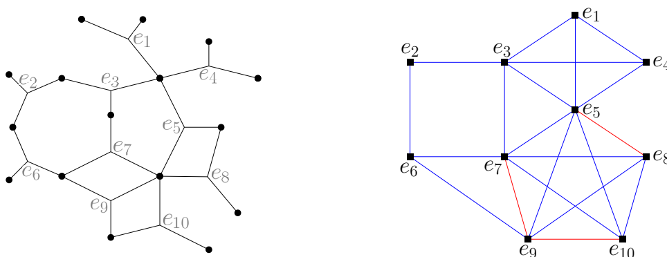
Figure 18: On the left: a 3-uniform hypergraph \mathcal{H} . On the right: the bicolored graph G = \varphi_{3,1}(\mathcal{H}) .
