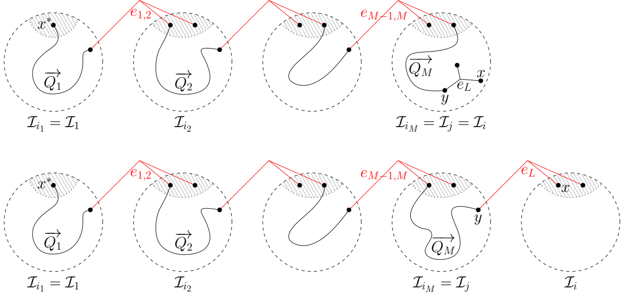
Figure 11: Top: e_L \in E(\mathcal{I}_i) . Bottom: e_L \notin E(\mathcal{I}_i) .
