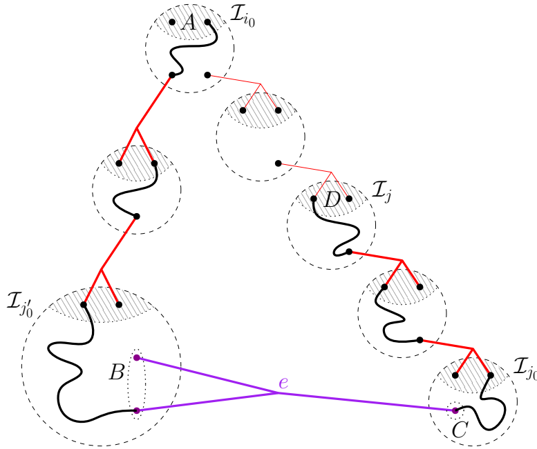
Figure 17: Illustration of Case 4 from Proposition 3.9. The bold paths (in red and black) are \vec{P} on the right and \vec{Q} on the left.
