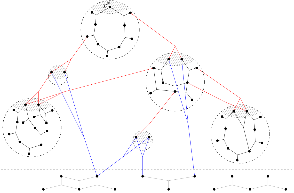
Figure 13: The hypergraph \mathcal{H} is represented in full. In black and red: E(\mathcal{A}) (archipelago). In blue: E_{cut} . In grey, below the dashed line: E_{ext} .
