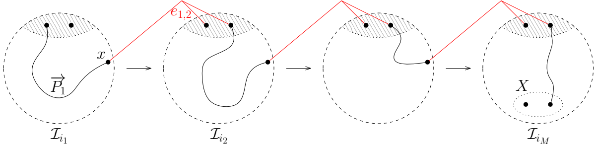
Figure 12: An (\varepsilon_{i_1}, X) -extendable path in an archipelago.
