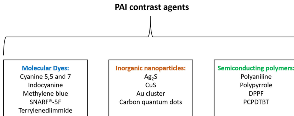
FIGURE 3 PAI contrast agents for multimodal cancer theragnostic and cancer hallmark imaging. SNARF®, seminaphtharhodafluor; DPPF, poly[3-(5-(9-hexyl-9-octyl-9H-fluoren-2-yl)thiophene-2-yl)-2,5-bis(2-hexyldecyl)-6-(thiophene-2-yl)pyrrolo[3,4-c]pyrrole-1,4(2H,5H)-dione]; PCPDTBT, poly[2,6-(4,4-bis(2-ethylhexyl)-4H-cyclopenta[2,1-b;3,4-b']dithiophene)-alt-4,7(2,1,3benzothiadiazole)]
