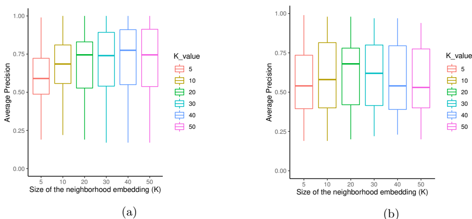
Figure 7: (a) The effect of parameter K on the AP (MPEG-7). (b) The effect of parameter K on the AP (Kimia99).
