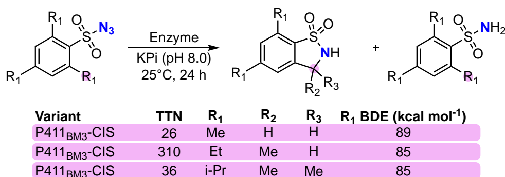
Scheme 7. C-H Amination of 2,4,6-Trialkyl-benzenesulfonyl azides producing benzosultam and arylsulfonamide.
