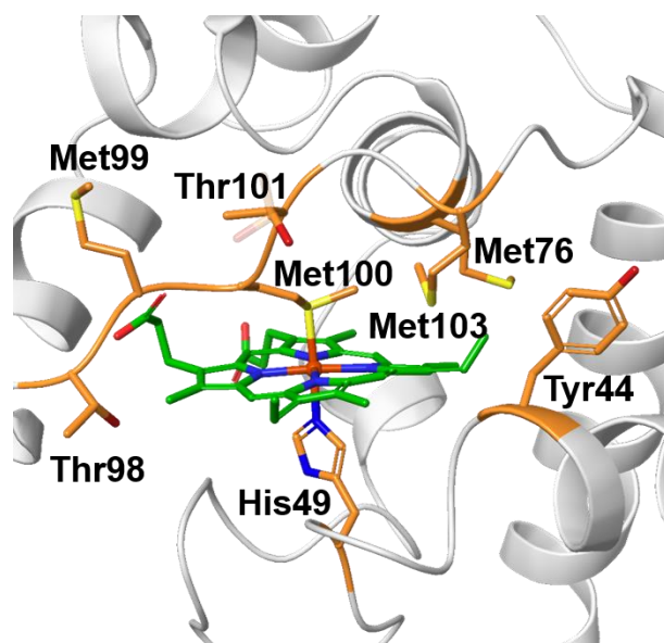
Figure 6. X-ray structure of the active site of Rma cytochrome c . Adapted from 84,87 with permission.
