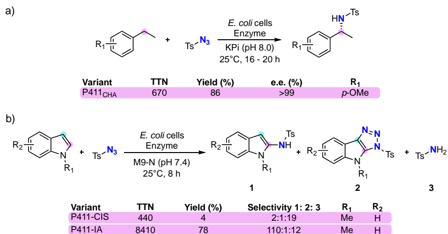
Scheme 11. Intermolecular aminations catalyzed by cytochrome P450 variants. 67,74
