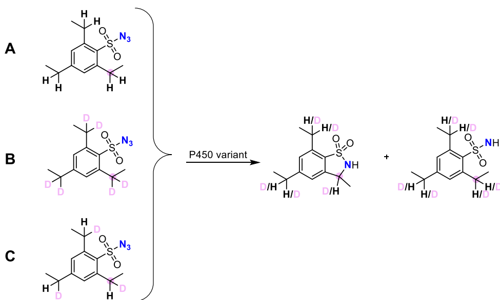
Fig. 3. Substrates used in Kinetic Isotope Effect experiments. 64 Experiment 1: the kinetic constants k_H and k_D of the reactions of A and B, respectively, were independently measured spectrophotometrically; experiment 2: the yields of the two products from the reaction of a 1:1 mixture of A and B were determined by ^1\text{H} NMR; experiment 3: the yields of the two products from the reaction of C were determined by ^1\text{H} NMR.
