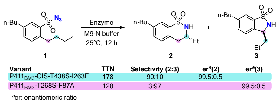
Scheme 8. Comparison of regioselectivities in benzosultam syntheses. 77 (er = enantiomeric ratio)
