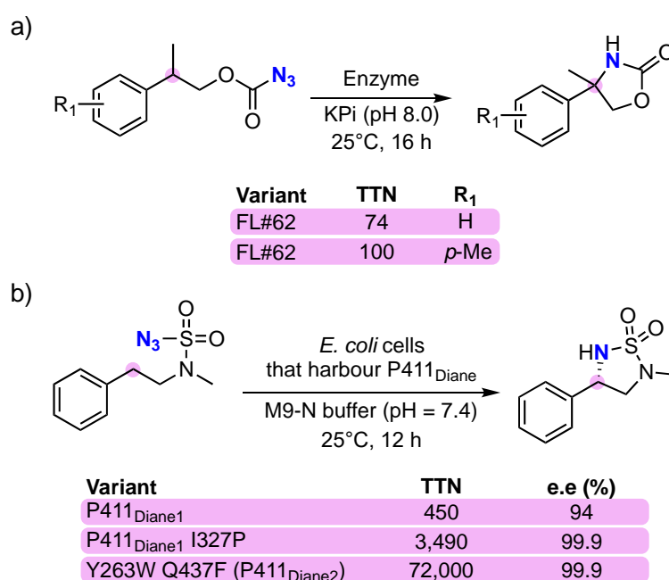
Scheme 9. Cyclization reactions catalyzed by enzymatic systems
