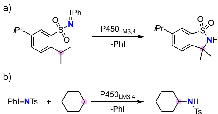
Scheme 3. In vitro enzymatic aminations by cytochrome P450 LM3,4 . 18
