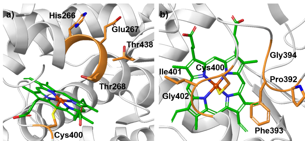
Fig. 2. Important residues in the heme distal (a) and proximal (b) regions of cytochrome P450 BM3 . Adapted from 64 with permission.
