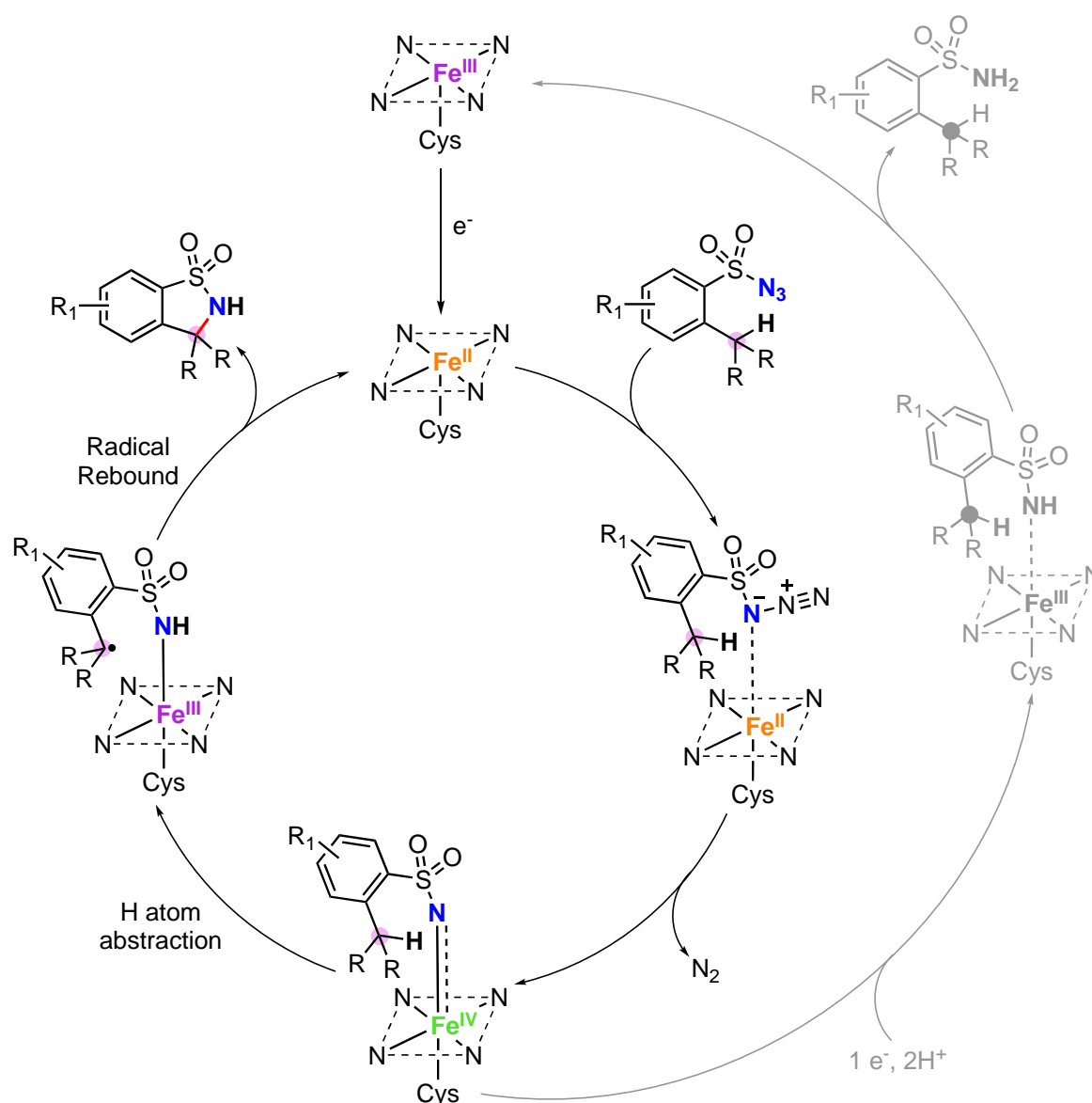
Fig. 4. Proposed mechanism for intramolecular C–H amination of sulfonyl azides catalyzed by cytochrome P450 and sulfonamide unproductive formation. Adapted from 64 with permission.
