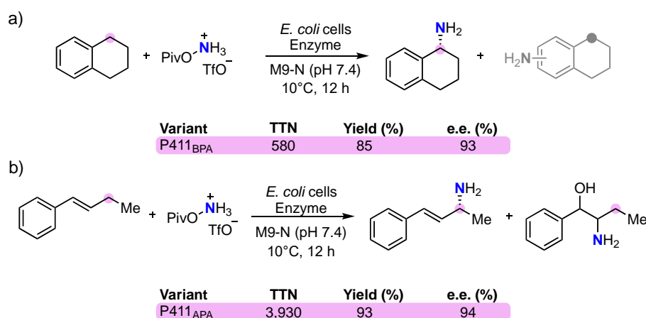
Scheme 12. Intermolecular primary aminations catalyzed by cytochrome P450 variants. 81 Reaction by-products are depicted in gray.
