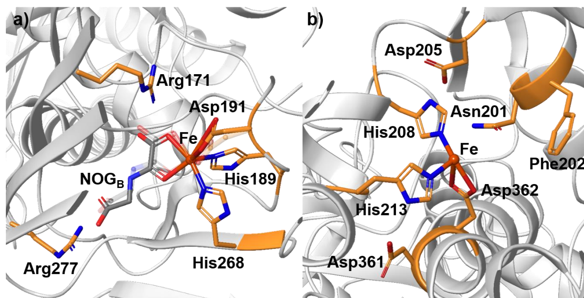
Figure 7. X-ray structures of the active sites of (a) Pseudomonas syringae pv. phaseolicola PK2 ethylene-forming enzyme 96 and (b) Escherichia coli naphthalene dioxygenase. 97 Adapted with permission.
