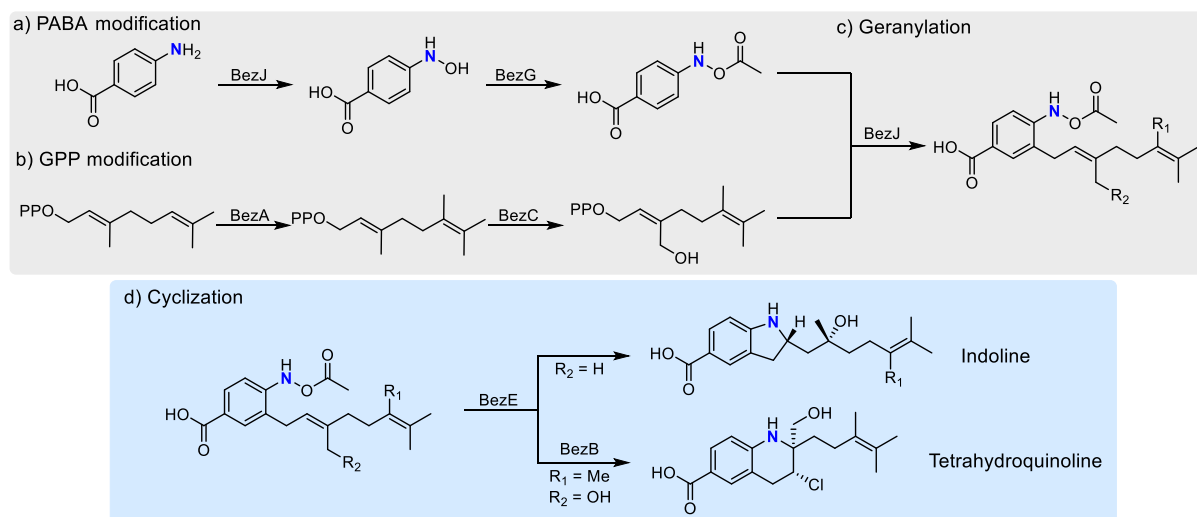
Scheme 4. Proposed biosynthesis of some benzastatins illustrating the principal enzymatic steps: (a) acetoxylation of PABA, (b) modification of geranyl pyrophosphate, (c) geranylation of modified PABA and (d) nitrene transfer and cyclization. Adapted from 25 with permission.
