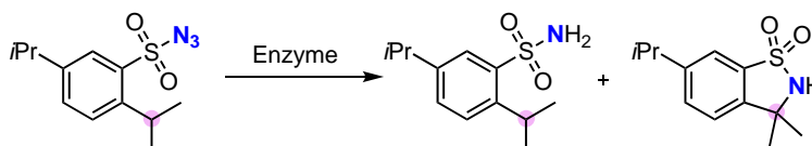
Scheme 6. Intramolecular amination forming the arylsulfonamide and the benzosultam.
