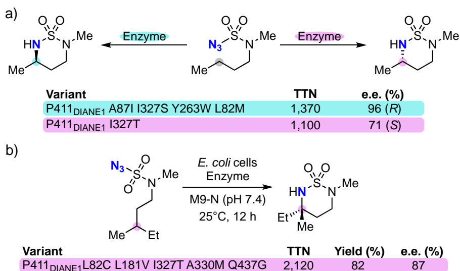
Scheme 10. Cyclization reactions catalyzed by cytochrome P450 variants 79
