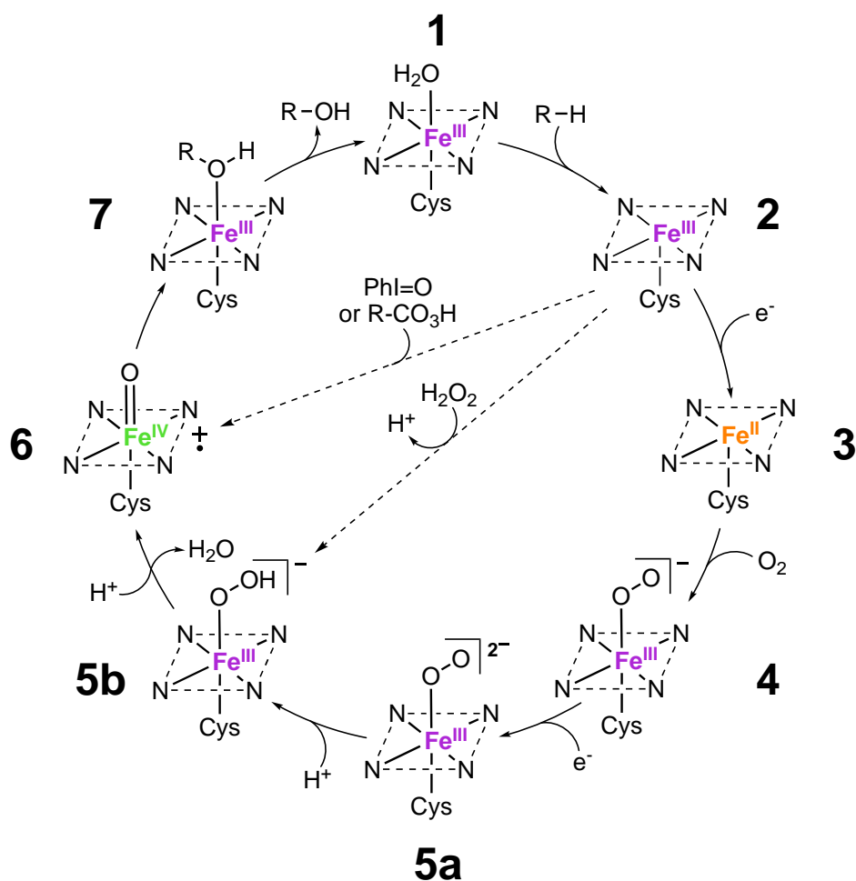
Fig. 1. Catalytic cycle of cytochrome P450. Adapted from 36 with permission.
