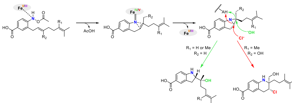
Scheme 5. Proposed mechanisms for aziridination and cyclization leading (with assistance of a protic residue) to indoline (green pathway) and tetrahydroquinoline (red pathway). Adapted from 25 with permission.
