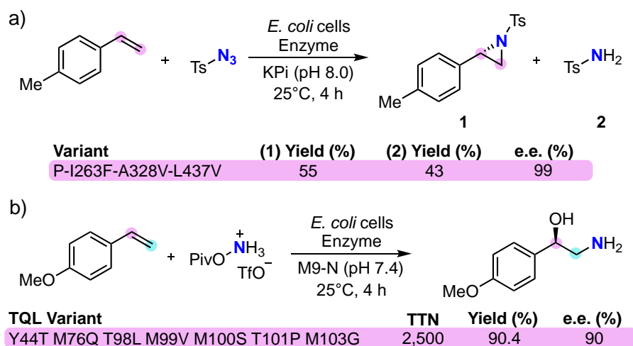
Scheme 14. a) p -Methylstyrene aziridination and arylsulfonamide formation (a) and p -methoxystyrene aminohydroxylation (b) catalyzed by cytochrome P450 variants.
