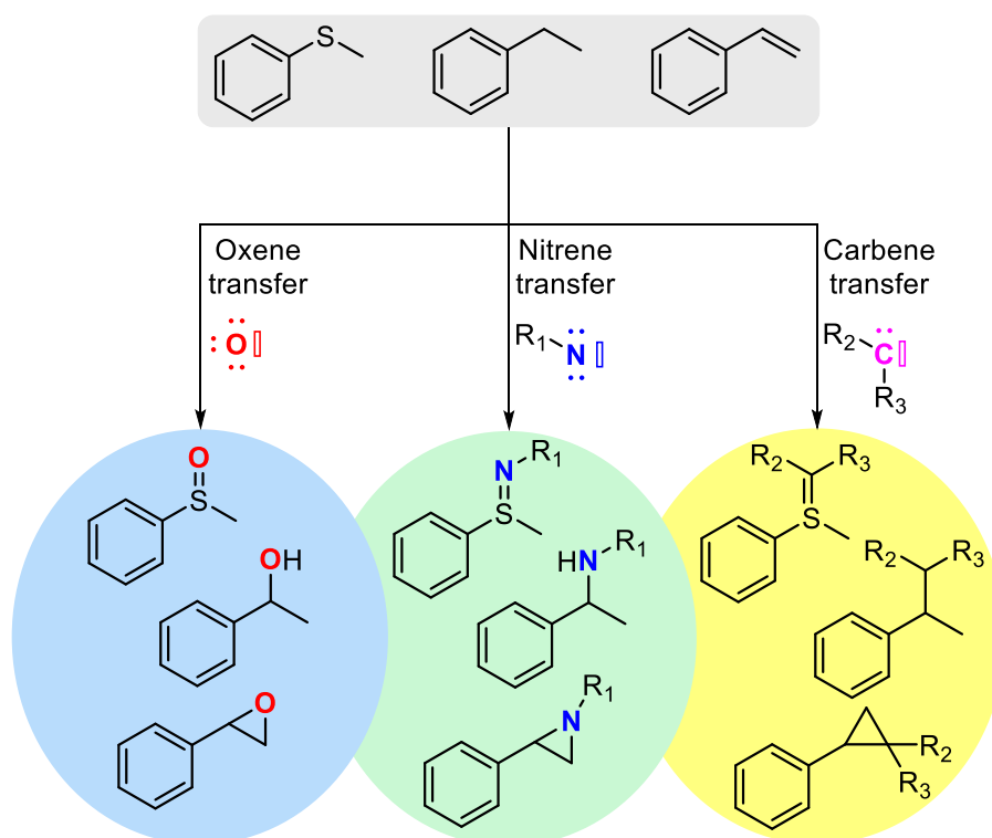
Scheme 1. Examples of oxene, nitrene and carbene transfers on representative phenyl derivatives.
