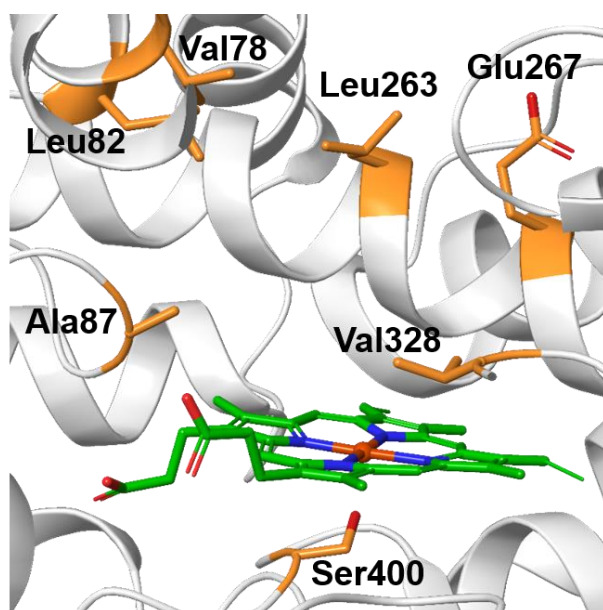
Figure 5. X-ray structure of the cytochrome P411 A82L A78V F263L variant showing important amino acids. Adapted from 74 with permission.
