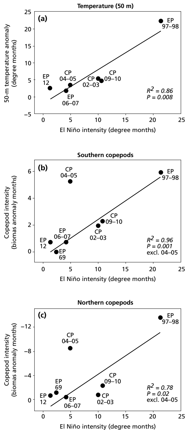
FIGURE 6.8 Relationship of El Niño intensity measured by the average of the SST anomalies in the Niño-3.4 region multiplied by the number of months that those anomalies were >0.5\text{ }^{\circ}\text{C} (degree months) vs. the (a) 50 m temperature anomaly (b) southern and (c) northern copepod intensity measured as the average temperature or biomass anomalies multiplied by the number of months when positive temperature anomalies ( >0.25\text{ }^{\circ}\text{C} ) or positive (negative) biomass anomalies of warm (cold) greater than (less than) 0.1\text{ mg C m}^{-3} were observed for two consecutive months at NH 5 ( 44.6\text{ }^{\circ}\text{N} ). SST, sea-surface temperature
