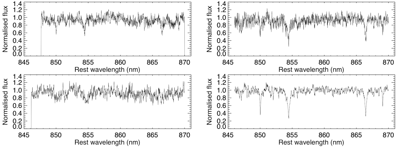
Fig. 3. Normalised RVS spectra, Doppler shifted to rest, resampled and combined into a single spectrum: S1 (left panels), S2 (right panels) from the CU6 pipelines: DR2 (top panels) and DR3 practice run (bottom panels) to show how deblending reveals S1’s uncontaminated spectrum in the bottom left panel. The number of combined CCD spectra are 21 (top left and top right), 26 (bottom left) and 43 (bottom right).
