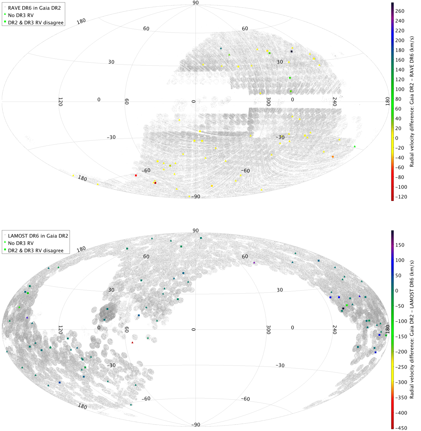
Fig. 26. Galactic Aitoff projection of RAVE DR6 ( top ) and LAMOST DR6 ( bottom ) stars in Gaia DR2, both colour-coded according to their respective radial velocity differences.
