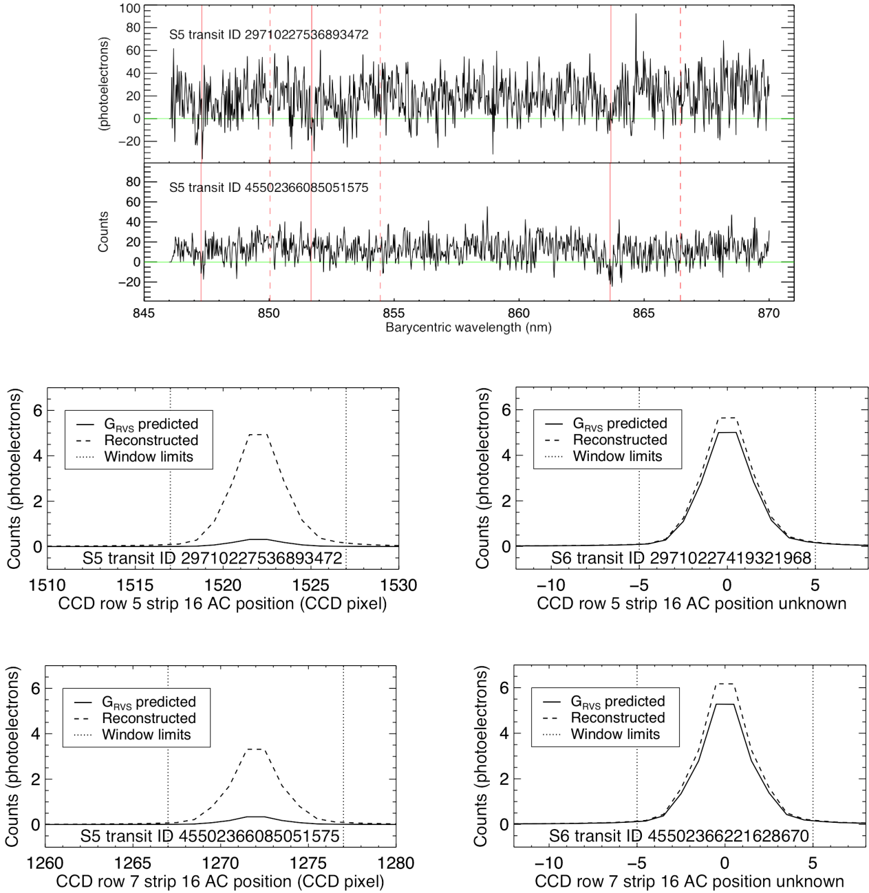
Fig. A.3: DR2 transits of S5. Top plot : the two DR2 transit (three-CCD averaged) spectra of S5. The red dashed lines delineate the Ca II absorption line rest wavelengths. The red solid lines are the aforementioned rest wavelengths, Doppler shifted according to the transit radial velocity. G_{RVS} -predicted and reconstructed AC profiles of S5 and S6 in the first transit ( middle two plots ) and the second transit ( bottom two plots ). S6 was processed by the CU6-DR3 pipeline, but the two transits closest in time to S5’s two transits were excluded because it could not be successfully deblended. Consequently, its window geometry information was not recorded, meaning its relative AL and AC positions and AC decentring are not known exactly. S5’s AC decentring is not known either because AC decentring is calculated in the CU6-DR3 pipeline and S5 was not processed by the CU6-DR3 pipeline. Consequently, the AC profiles in the middle and bottom panels are centred in the centre of their windows, but this may not be correct.
