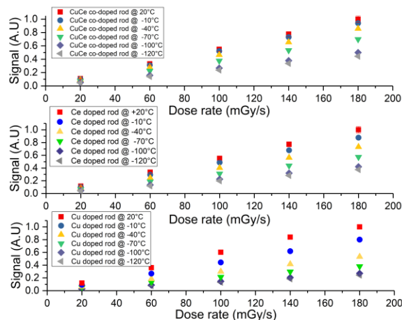
Fig. 3. Rods response measured by the PMT when varying the dose rate from 20 to 184 mGy/s at temperatures ranging from -120 °C to +20 °C. Error bars on the signal (y-axis) are smaller than the dots size.
