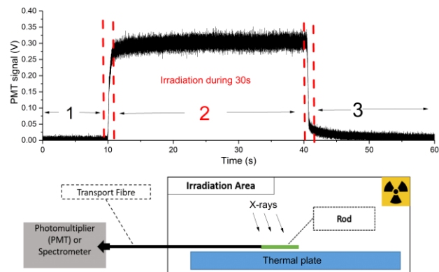
Fig. 1. (a) An example of a typical RIL measurement showing area 1 before irradiation, area 2 during irradiation at constant dose rate, and area 3 after irradiation. (b) Schematics of the experimental setup of the MOPERIX facility, and related acquisition equipment.
