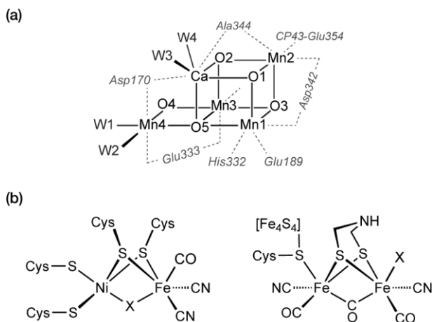
Scheme 1. (a) Structure of the \text{Mn}_4\text{CaO}_5 cluster in the active site of the OEC of photosystem II, showing standard atom labelling. W1–W4 represent water-derived ligands. (b) Structures of the active sites of the [NiFe] and [FeFe] hydrogenases, with X representing the site for catalytic \text{H}_2 /proton turnover.
