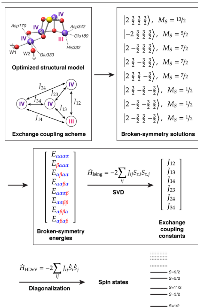
Figure 2. Flow diagram of calculations in the context of the broken-symmetry DFT approach for determining the exchange coupling constants and spin state ladder for a computational model of the S_2 state of the OEC, assuming Mn oxidation states of III-IV-IV-IV. Note that in this case there are only seven BS determinants that can be formed in addition to the high-spin determinant, yet the proper solution to the exchange coupling problem yields in total 320 states (including sublevels of spin multiplets).
