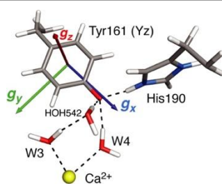
Figure 7. Orientation and components of the g -matrix for the S_2^B Y_2^* state according to Retegan et al. 182 with DFT-computed values g_x = 2.0054 > g_y = 2.0042 > g_z = 2.0022 . The immediate hydrogen bonding environment of the radical is also depicted.
