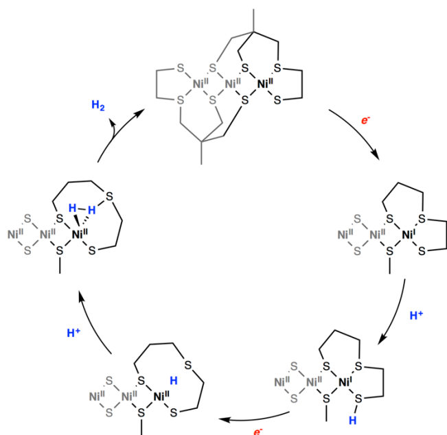
Figure 16. DFT computed reaction mechanism for hydrogen evolution mediated by a bio-inspired mimic for the [Ni-Fe] hydrogenase. Adapted with permission from Ref. 299. Published by The Royal Society of Chemistry.
