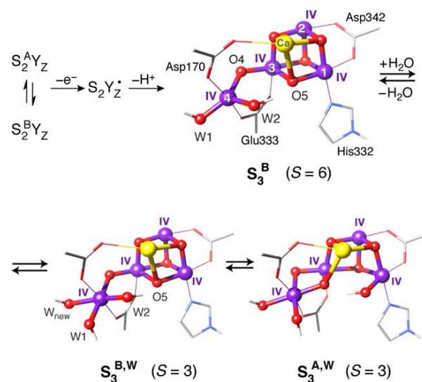
Figure 4. Possible structural components of the S_3 state of the OEC with their corresponding spin states.
