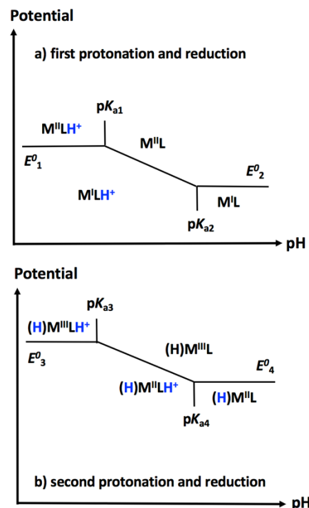
Figure 15. Representation of the Pourbaix diagram of a given catalyst based on a CECE sequence with MLH the ligand protonated species and (H)M the hydride intermediates. The horizontal lines are plotted with respect to the reduction potentials of the catalyst, while vertical lines are plotted for its pK_a values. Diagonal lines separate processes involving a simultaneous oxidation and protonation process.
