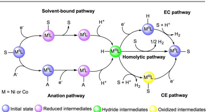
Figure 17. Examples of solvent-bound and anation reaction pathways to form hydride intermediates. Adapted with permission from Ref. 291. Copyright 2019 Chem Pub Soc.
