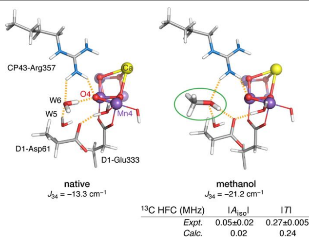
Figure 5. Proposed model for interaction of methanol with the OEC. 116 The increase in Mn3–Mn4 antiferromagnetic exchange coupling explains the stabilization of the low-spin S = 1/2 state of the cluster. The model is the only one of those examined that simultaneously agrees with the experimental ^{13}\text{C} hyperfine coupling parameters of Oyala et al. 167 Figure adapted from Ref. 116 – Published by The Royal Society of Chemistry.
