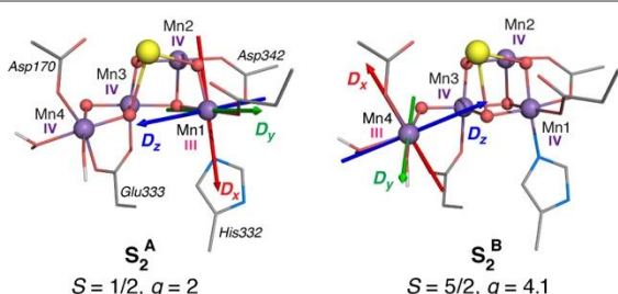
Figure 6. Orientation of principal axes of the D_{zOEC} for the five-coordinate Mn(III) ion in each isomer of the S_2 state of the OEC, computed with the L-CASCI approach. Adapted with permission from Retegan et al. 180 Copyright 2014 American Chemical Society.
