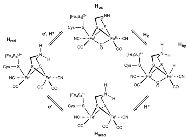
Figure 11. Postulated reaction mechanism of the [FeFe] hydrogenase involving the H ox , H hyd , H red , and H sred states.
