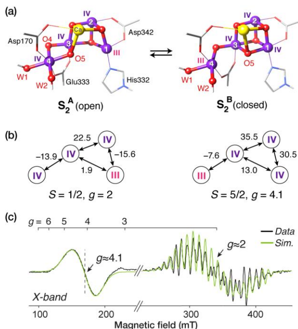
Figure 3. (a) Computational valence isomer models for the S_2 state of the OEC. (b) Computed nearest-neighbor exchange coupling constants and resulting spin states. (c) The valence isomers rationalize the two EPR signals associated with the S_2 state. In addition, they are very close in energy and interconvertible over a low barrier, as required experimentally, and they are each consistent with independent spectroscopic measurements for each g signal, including the ^{55}\text{Mn} hyperfine coupling constants and the distinct localization of the Mn(III) ion in each case.
