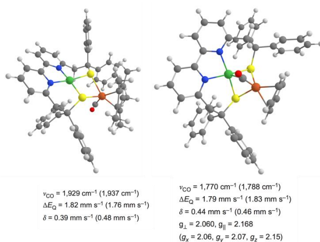
Figure 13. Structures of the biomimetic models for the Ni-S1a (a) and Ni-L (b) states of the [NiFe] hydrogenase identified by combining spectroscopic measurements and DFT computations. Adapted with permission from Ref. 40. Copyright 2016 Nature Publishing Group.
