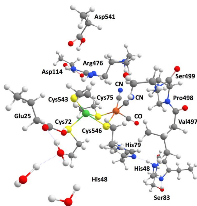
Figure 12. Example of a large model system including relevant amino acids and mimicking the active site of the [NiFe] hydrogenase.
