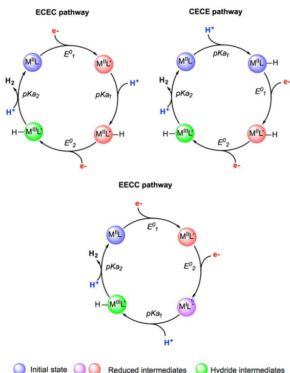
Figure 14. Selected examples of sequences and putative intermediates considered during hydrogen evolution reaction. Adapted with permission from Ref. 291. Copyright 2019 Chem Pub Soc.
