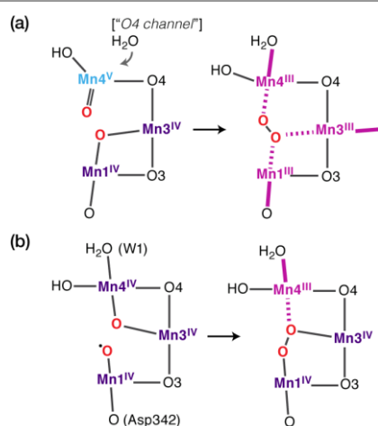
Figure 9. Schematic depiction of two possibilities for the O–O bond formation step in the S_4 state. (a) Creation of a Mn(V)=oxo species from a preceding water-unbound conformation of the S_3 state enables even-electron intramolecular nucleophilic coupling that resets the cluster to the S_0 oxidation state level. (b) Creation of a Mn(IV)-oxyl intermediate leads to radical oxyl–oxo coupling.
