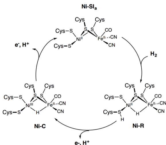
Figure 10. Proposed catalytic cycle of the [NiFe] hydrogenase involving the Ni-SI a , Ni-R, and Ni-C states.
