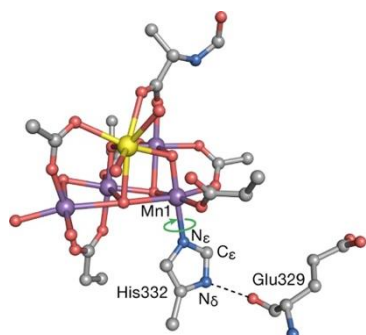
Figure 8. The His332–Glu329 hydrogen bonding interaction constrains the imidazole plane of the histidine residue. Computational models that do not take this into account lead to incorrect description of the coordination sphere of Mn1 and all processes and properties associated with it. Adapted with permission from Ref. 193. Copyright 2013 American Chemical Society.
