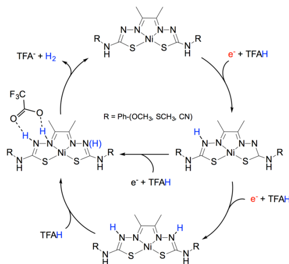
Figure 18. DFT computed reaction mechanism for hydrogen evolution mediated by a molecular catalyst highlighting the influence of the proton source on the preferable pathway. Adapted with permission from Ref. 309. Published by The Royal Society of Chemistry.
