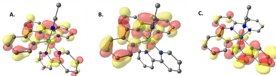
Figure 3. Localized SOMOs for (A) the one-electron reduced complex 1-MeCN -1 and (B-C) the two-electron reduced complex 1-MeCN -2 .
