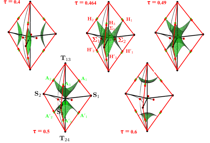
Fig. 7 \tau -surfaces in the three dimensional composition space. The \tau -surfaces are hyperboloids with three sheets for \tau < 2\sqrt{3} - 3 \approx 0.464 , a single sheet for 2\sqrt{3} - 3 < \tau < 1/2 , and two sheets for 1/2 < \tau < 1 . The special points in green, \mathbf{O} , \mathbf{A}_1 , \mathbf{A}_2, \dots for \tau = 0.5 , and the special points in red \Sigma_1 , \Sigma_2 , \Sigma_3 , \mathbf{H}_1 , \mathbf{H}_2, \dots for \tau = 0.464 are the same as in Fig.6.
