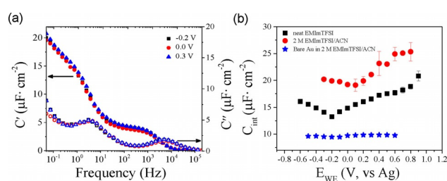
Figure 1. Capacitance change of a SLG electrode in diluted ionic liquid electrolyte. a) Real part and imaginary parts of electrochemical capacitance ( C and C' , respectively) of SLG with respect to the applied frequency, measured at different potentials in 2 M EMImTFSI/ACN. b) C_{\text{int}}-E curves of SLG in neat ionic liquid and ionic liquid dissolved in ACN electrolytes, where C_{\text{int}} is the interfacial capacitance of the SLG electrode obtained from the extrapolation.
