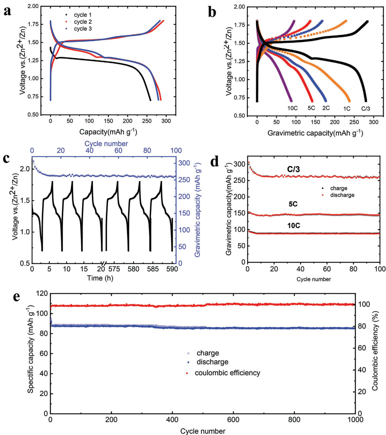
Figure 3. Electrochemical characterization of \text{K}_{0.27}\text{MnO}_2 \cdot 0.54\text{H}_2\text{O} in 2 M \text{ZnSO}_4 + 0.3 M \text{MnSO}_4 electrolyte. a) Galvanostatic charge/discharge profiles of the first three cycles at C/3. b) Discharge–charge curves at various C-rates. Cycling performance at a current density of c) C/3 and e) 10C. d) Comparison of cycling stability of first 100 cycles at C/3, 5 C, and 10 C.
