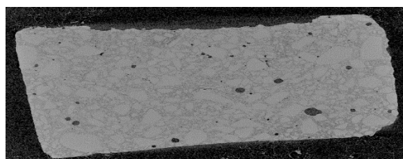
Figure 3. Tomography (internal diameter cut view, diameter: 10 mm) of the sample consolidated by freeze isostatic pressure (FIP) showing a non-uniform distribution of pores and inhomogeneous repartition of solvent (presence of agglomerates).
