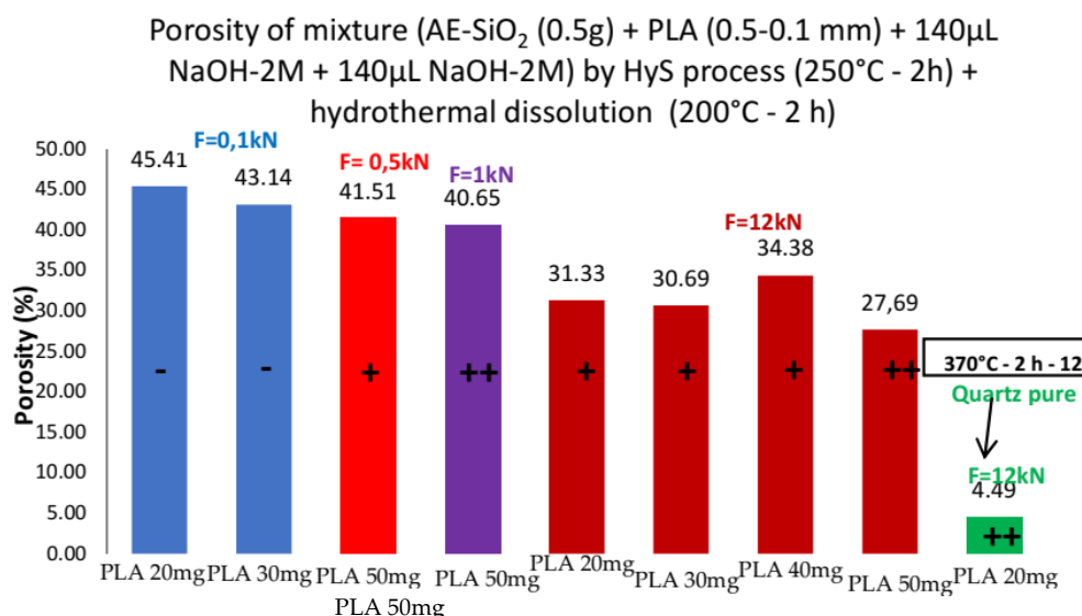
Figure 6. Porosity of AE SiO 2 by hydrothermal dissolution.
