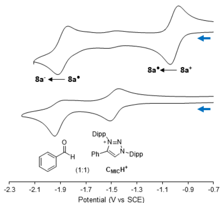
Figure 5: Cyclic voltammograms of compound 8a•BF 4 (up) and a 1:1 mixture of tetrafluoroborate salt of C MIC • H + and benzaldehyde (down) (1 mM solution employing 0.1 M of nBu 4 NPF 6 in acetonitrile electrolyte; 100 mV/s rate, for both cases).
