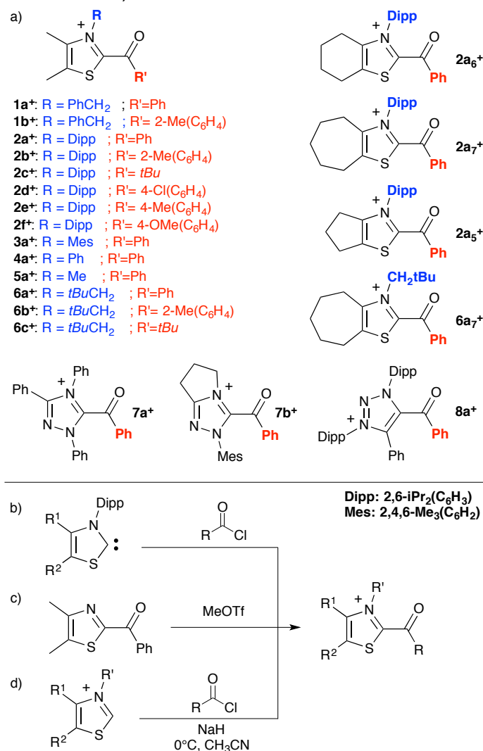
Scheme 1: (a) Structure of acyl azoliums 1 + -8 + ; synthesis of acyl thiazolium by: (b) acylation of persistent carbenes, (c) alkylation of an acyl thiazole or (d) in situ trapping of transient carbenes with acyl chlorides.
