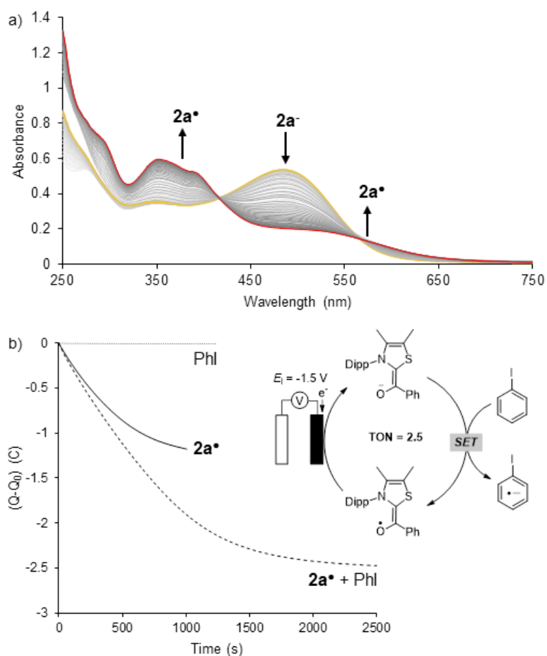
Figure 4: (a) UV-vis monitoring of the reaction of 2a^- (1 mM) with iodobenzene (2 mM). (b) Coulometric monitoring of electrolyses of 2a^\cdot (1 mM) and/or PhI (20 mM) at -1.5 V versus SCE.
