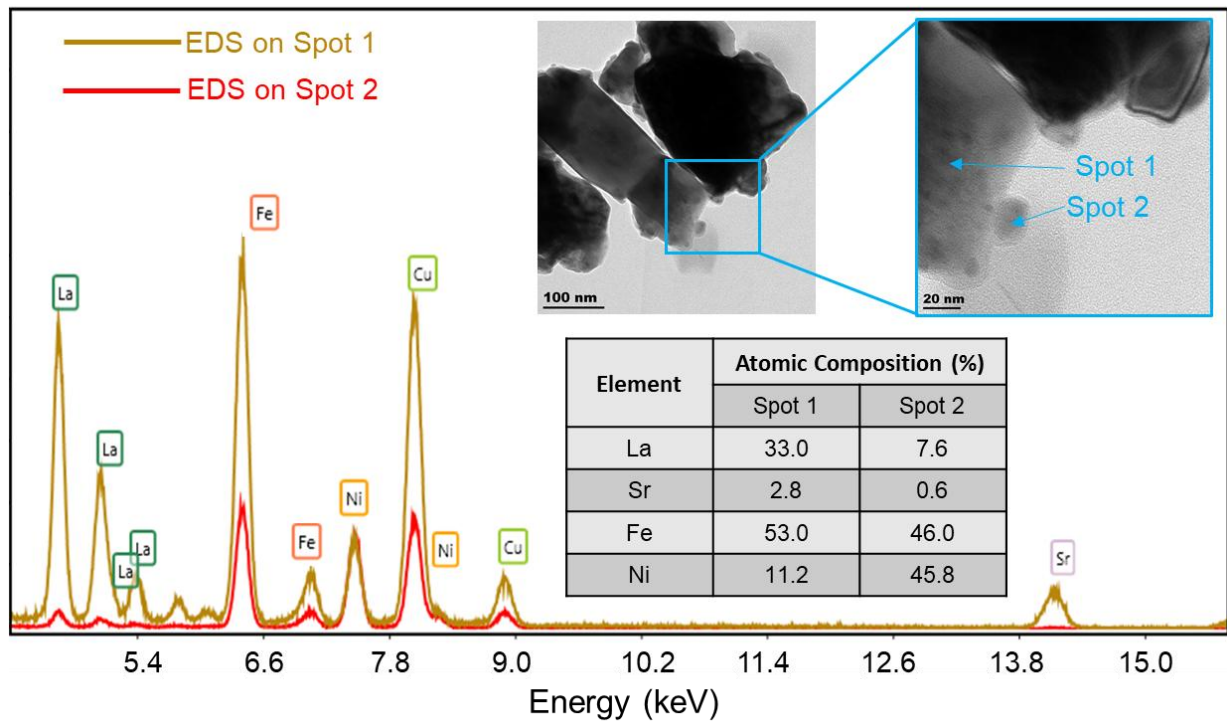
Figure 9: Energy dispersive spectra of LSNF treated under 5% H_2/N_2 at 800 °C for 2 hours collected at two different spots. Spot 1 was from the perovskite structure near to a nanoparticle and spot 2 was from the nanoparticle.
