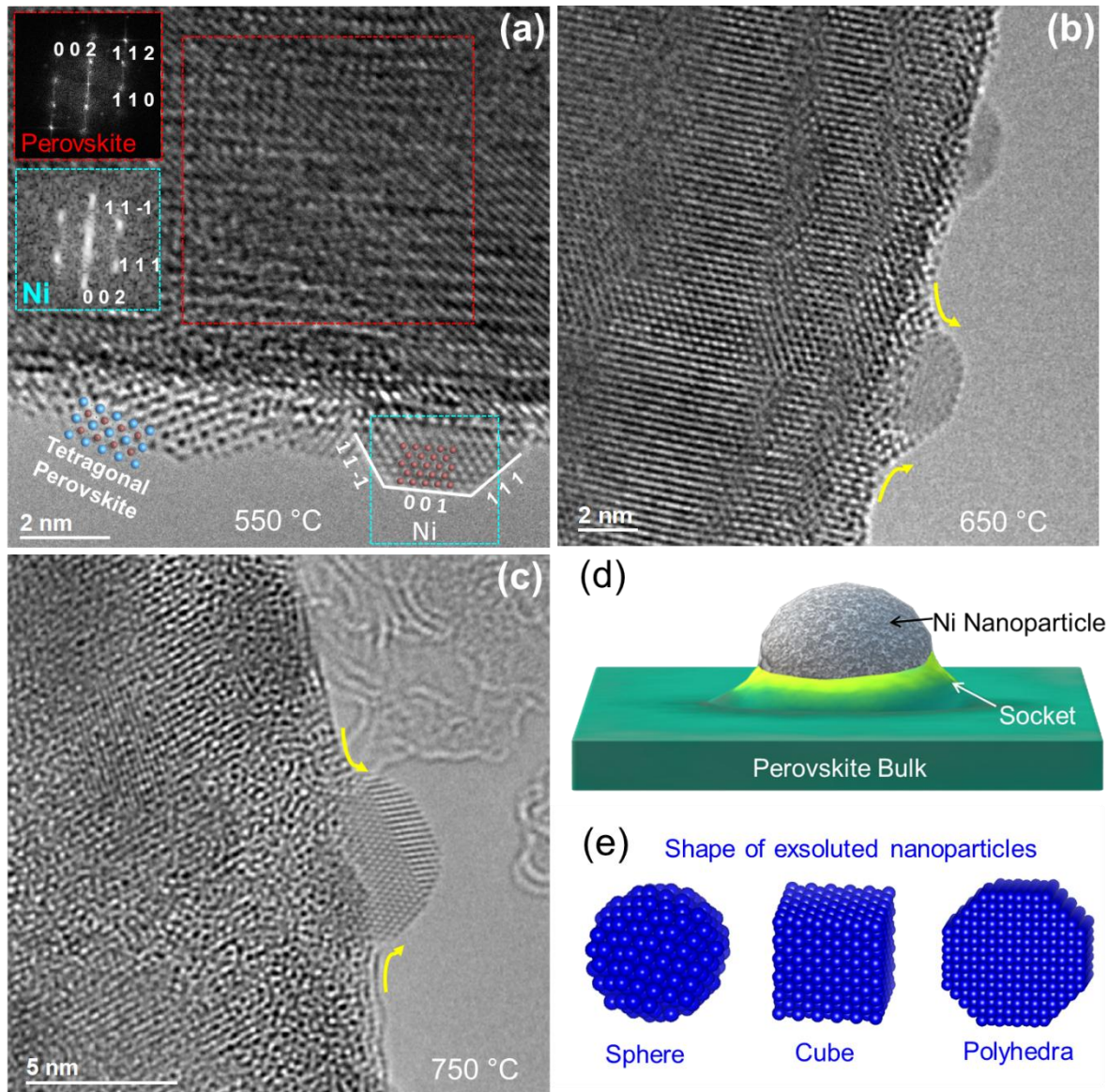
Figure 7: In-situ TEM of LSNF under 5% H 2 /N 2 collected at (a) 550 °C, (b) 650 °C, (c) 750 °C showing formation of a socket around the nanoparticle. (d) a schematic illustration of socket formation around a nanoparticle, (e) a schematic illustration of various shapes observed for the nanoparticles.
