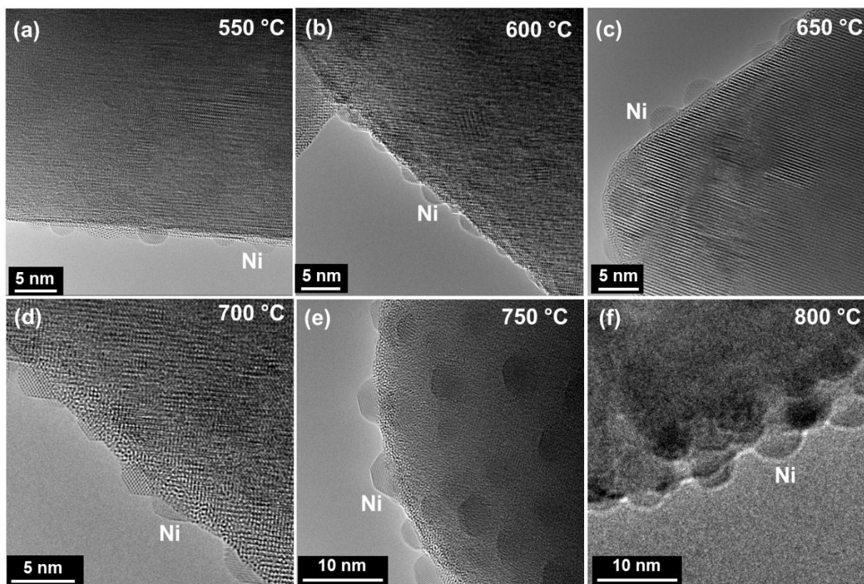
Figure 6: In-situ TEM of LSNF under 5% H 2 /N 2 collected at (a) 550 °C, (b) 600 °C, (c) 650 °C, (d) 700 °C, (e) 750 °C, and (f) 800 °C.
