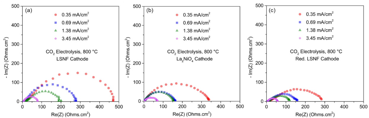
Figure 17: EIS collected at various current densities during electrolysis of CO 2 at 800 °C.
