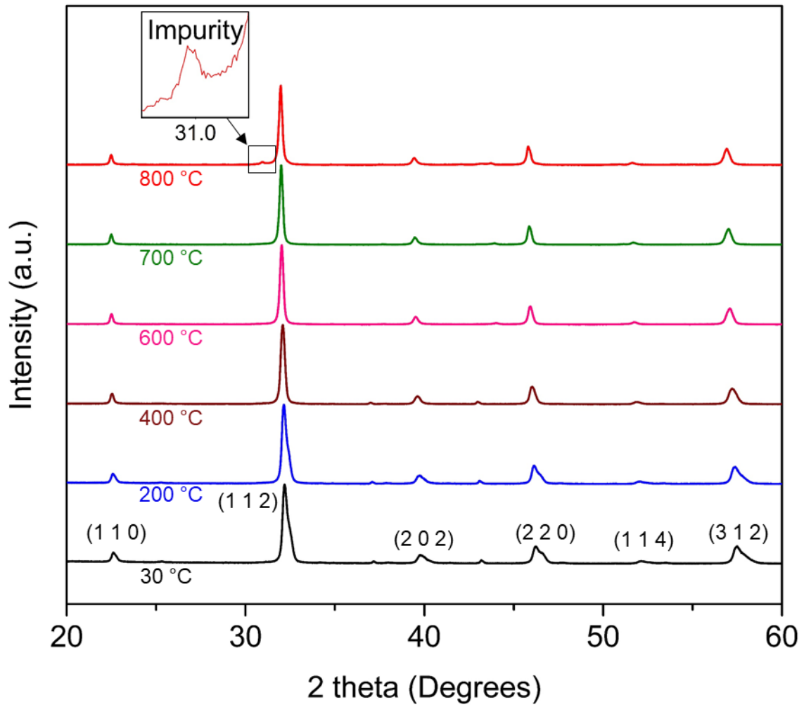
Figure 2: In-situ XRD of LSNF under 5% H 2 /N 2 at different temperatures.
