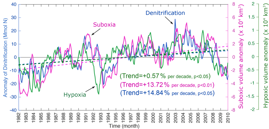
Figure 5. Changes in oxygen minimum zone and denitrification in the northern AS. Interannual anomalies in the volume of suboxia (purple), hypoxia (green) and water column denitrification (blue) in the upper 1000 m north of 20° N over the study period. The dashed lines indicate the trend lines. The location of the northern AS box is shown in Fig. 4a.
