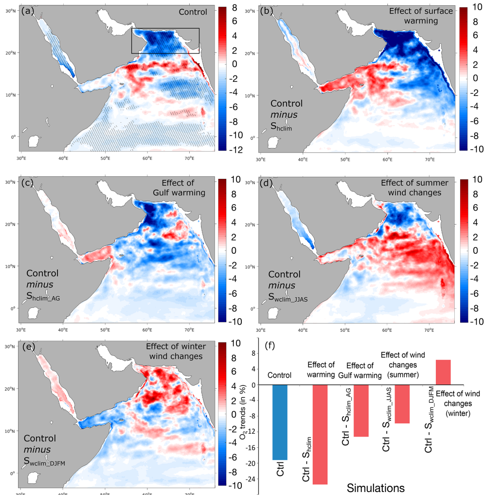
Figure 8. Effects of different atmospheric forcing perturbations on deoxygenation rates. (a) Linear trends in O 2 inventories in the 100–1000 m layer in the control run (in percent per decade). (b–e) Difference in O 2 inventory trends between the control run and the S_{hclim} (i.e., effect of warming), S_{hclim\_AG} (i.e., effect of Gulf warming), S_{wclim\_JJAS} (i.e., effect of summer wind intensification) and S_{wclim\_DJFM} (i.e., effect of winter wind changes) sensitivity simulations in the 100–1000 m layer (in percent per decade). (f) Difference in O 2 inventory trends in the northern AS box between the control and the different sensitivity simulations (in percent of the mean O 2 inventory over the 1982–2010 period).
