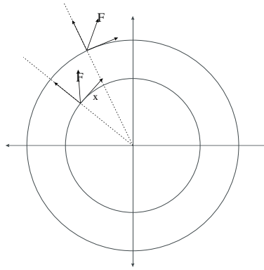
Figure 3: Summation of the forces applied to two-dimensional objects result in a rotation about the center of the expanding sphere.
