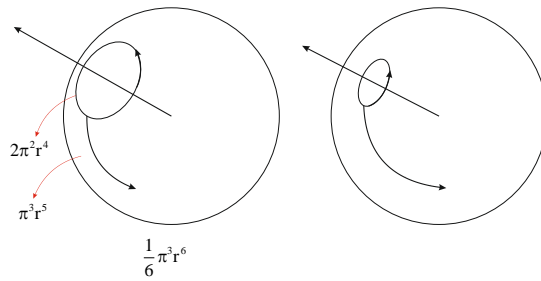
Figure 8: When a mass gains velocity, the oscillation radius becomes smaller in higher dimensions.
