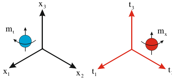
Figure 12: The relative mass is created from motion in space, while the particle's mass is due to motion in time. The particles' characteristics other than mass, including spin, load and Polarization have two different states in space and time, as well.
