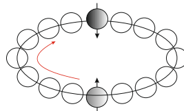
Figure 13: If a particle with a spin along the z-axis rotates about the center of circle with a high velocity, the particle's spin due to its own magnetic field, creates different cases in different points of the circle with respect to the z-axis.
