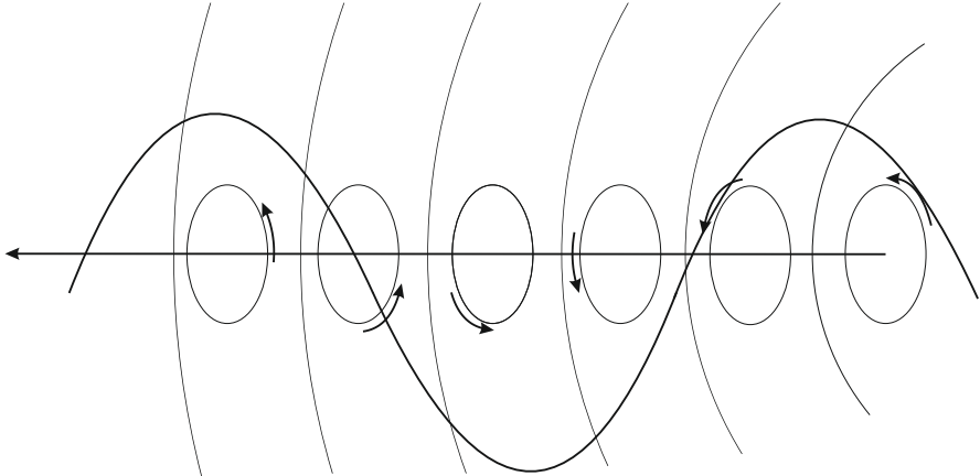
Figure 14: An object is moving in space and time in a four-dimensional space (the circumference of a small circle). With the expansion of the five-dimensional sphere and the displacement of the object in the space-time, a wave is created the wavelength of which is equal to the wave attributed to the matter.
