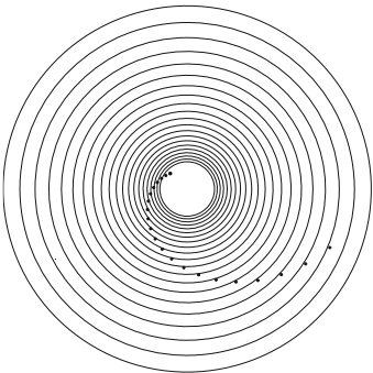
Figure 15: The movement of objects in the time dimension in form of logarithmic spiral based on the golden ratio.
