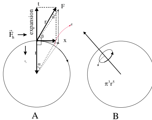
Figure 6: The summation of the forces on the surface of the sphere and the resistance force of the expanding sphere result in the rotation of two-dimensional spots of the sphere surface about the center of the sphere. B: In the six-dimensional space, three imaginary vectors exist for the three-dimensional world on the surface of curved four-
