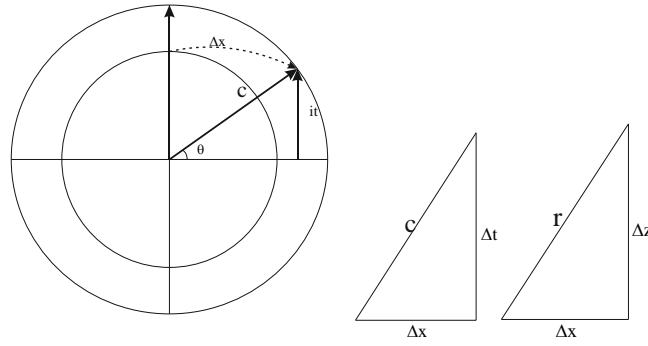
Figure 2: If r is considered as the speed of light and x denotes the speed of the movable, the z dimension represents the imaginary dimension of time for all points on the surface of the sphere, and the sine of the angle \theta , represents the amount of the movable's eccentricity from the time arrow axis.
