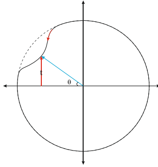
Figure 17: Each mass can be considered equivalent to a length in space and time and density causes a curvature in expanding space-time and thus time passes slower in the gravitational field.
