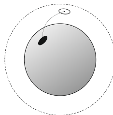
Figure 1: every motion on the surface of an expanding sphere, has a relative motion with regards to the z-axis, and the path of the movable in the three-dimensional space is a curved path.
