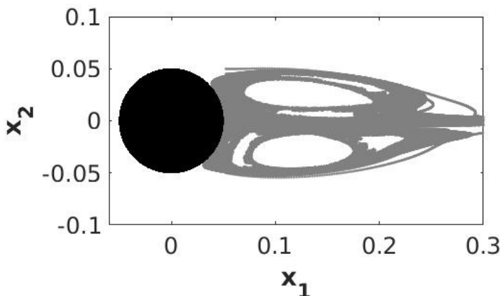
Figure 7: Streakline experiment for the ROC system with injection points at \mathbf{p} = (x_1, x_2) / x_1 = 0.0525; x_2 \in [-0.05 : 0.005 : 0.05] . The picture corresponds to the instant t = 125 T_p(\text{ROC}) . The dye (in gray) never invades the circular and triangular regions.
