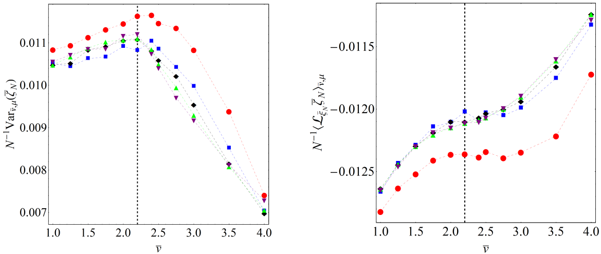
Figure 5. Quantites entering Eq.(39) for lattices with different N . In particular, N = 400 (blue squares), N = 900 (black diamonds), N = 1600 (green triangles), N = 2500 (purple reversed triangles).
