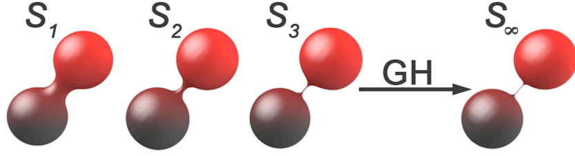
Figure 4. Sequence of diffeomorphic manifolds (of the same dimension) with a limit manifold which is not diffeomorphic to the members of the sequence. The infinitely tiny bridge between the two spheres of S_\infty has infinite mean curvature.
