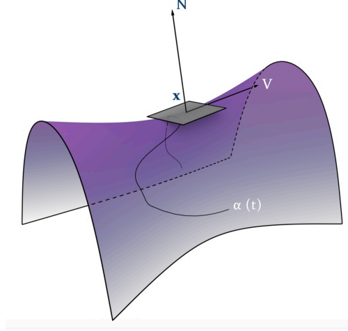
Figure 3. Illustration of the ingredients necessary to construct the shape operator of a surface.
