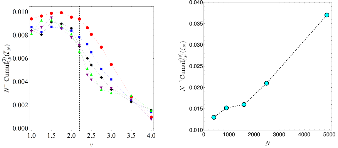
Figure 8. Quantities entering Eq.(39) for lattices with different N . Left panel: third cumulant of \bar{\zeta}_N for N = 400 (blue squares), N = 900 (black diamonds), N = 1600 (green triangles), N = 2500 (purple reversed triangles). Right panel: fourth cumulant of \bar{\zeta}_N computed at the transition energy density \bar{\nu}_c \simeq 2.2 , here a systematic deviation from the gaussian scaling with N is well evident.
