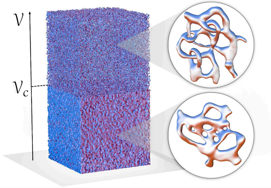
Figure 1. Low-dimensional pictorial representation of the transition between complex topologies as a metaphor of the origin of a phase transition. From the ground level up to the crossover level v_c , the manifolds M_v have a genus which increases with v . Above the crossover level v_c , the manifolds M_v have also a nonvanishing linking number which increases with v
