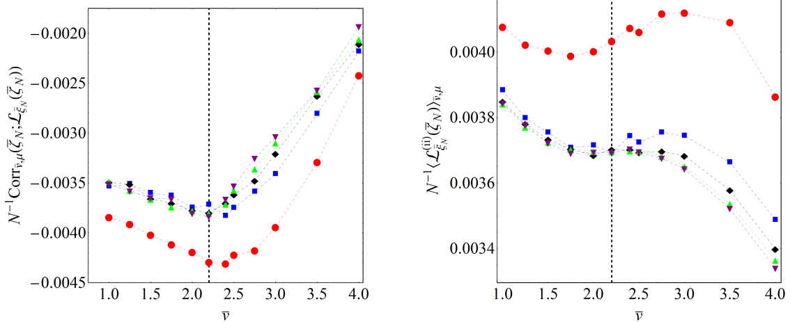
Figure 6. Quantities entering Eq.(39) for lattices with different N . In particular, N = 400 (blue squares), N = 900 (black diamonds), N = 1600 (green triangles), N = 2500 (purple reversed triangles).
