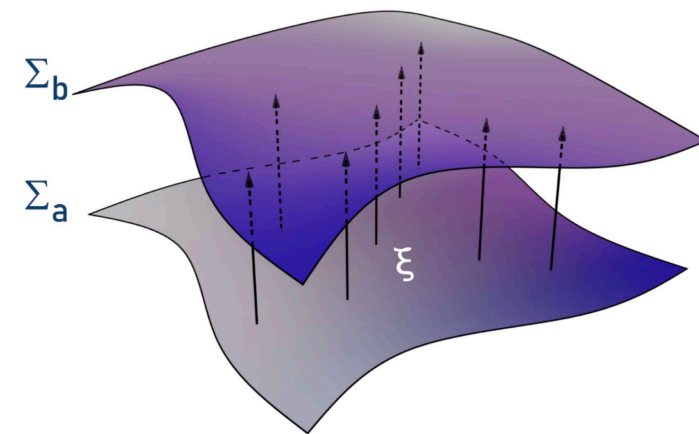
Figure 2. Pictorial representation of the action of the vector field \boldsymbol{\xi} in Eq.(2) diffeomorphically mapping each point of the level set \Sigma_a onto each point of the level set \Sigma_b .
