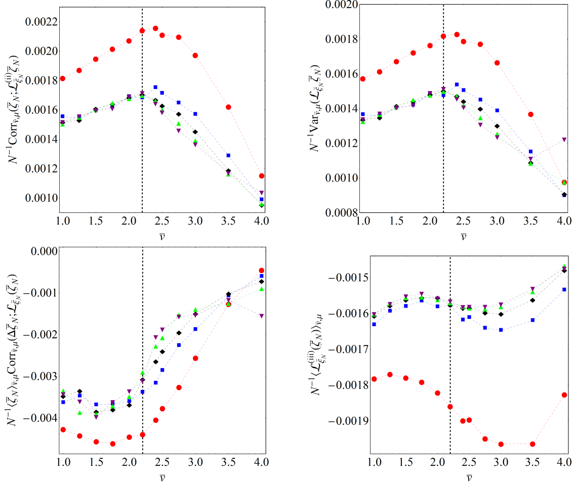
Figure 7. Quantites entering Eq.(39) for lattices with different N . In particular, N = 100 (red full circles), N = 400 (blue squares), N = 900 (black diamonds), N = 1600 (green triangles), N = 2500 (purple reversed triangles).
