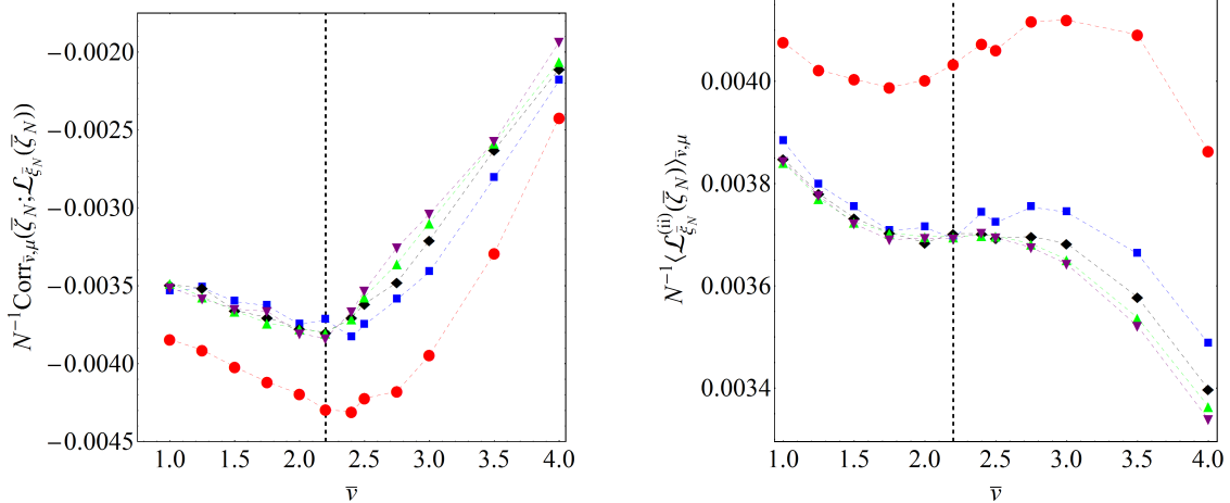
Figure 6. Quantities entering Eq.(39) for lattices with different N . In particular, N = 100 (red full circles), N = 400 (blue squares), N = 900 (black diamonds), N = 1600 (green triangles), N = 2500 (purple reversed triangles).
