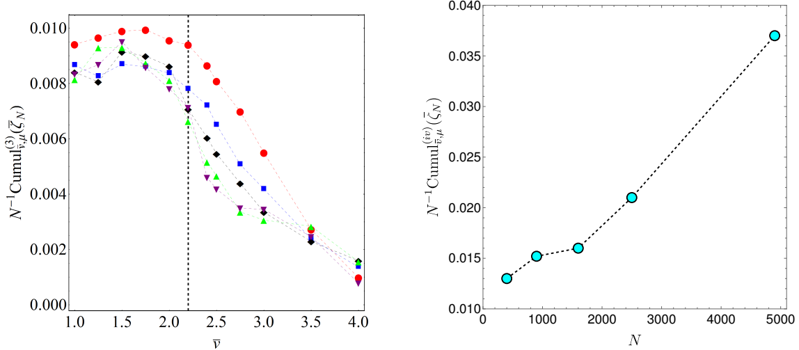
Figure 8. Quantites entering Eq.(39) for lattices with different N . Left panel: third cumulant of \bar{\zeta}_N for N = 100 (red full circles), N = 400 (blue squares), N = 900 (black diamonds), N = 1600 (green triangles), N = 2500 (purple reversed triangles). Right panel: fourth cumulant of \bar{\zeta}_N computed at the transition energy density \bar{\nu}_c \simeq 2.2 , here a systematic deviation from the gaussian scaling with N is well evident.
