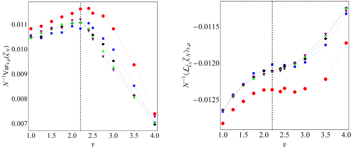
Figure 5. Quantites entering Eq.(39) for lattices with different N . In particular, N = 100 (red full circles), N = 400 (blue squares), N = 900 (black diamonds), N = 1600 (green triangles), N = 2500 (purple reversed triangles).
