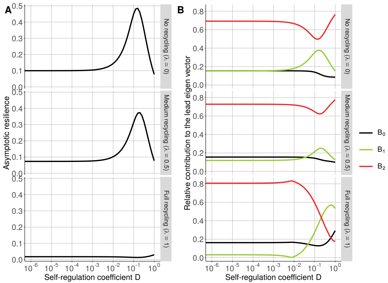
Figure S2-6: Linear stability depending on recycling efficiency \lambda and self-regulation coefficient D in a food chain with a chain length equal to 2 (TL2). A) Asymptotic resilience (opposite of the real part of the lead eigen value of the Jacobian matrix of the system at equilibrium). B) Relative contribution of each compartment to the lead eigenvector.
