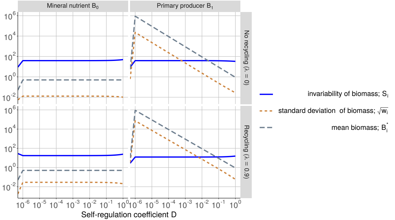
Figure S2-7: Stability of the different compartments depending on the recycling efficiency \lambda and the self-regulation coefficient D in a food chain with a chain length equal to 1 (TL1). Stability is measured by the invariability ( i.e. , inverse of CV), the ratio between equilibrium B_i^* and the standard deviation \sigma_i . The parameter I is fixed to 0.05.
