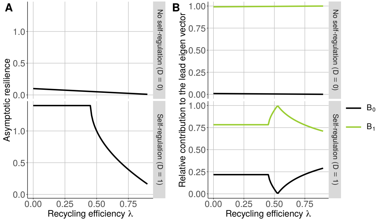
Figure S2-1: Linear stability depending on recycling efficiency \lambda and self-regulation coefficient D in a food chain with a chain length equal to 1 (TL1). A) Asymptotic resilience (opposite of the real part of the lead eigen value of the Jacobian matrix of the system at equilibrium). B) Relative contribution of each compartment to the lead eigen vector.
