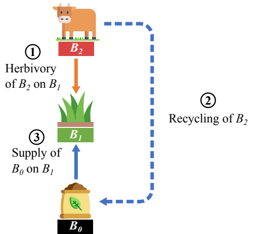
Figure 7: Schematic representing the direct and indirect effects of A ) herbivores on mineral nutrients. Blue arrows represent the positive terms (2) \lambda(m + 2DB_2) + \lambda(1 - b_2)a_2B_1 , (3) \lambda(m + 2DB_1) + \lambda(1 - b_2)a_2B_2 . Orange arrows represent the negative terms (1) -a_2B_1 and (3) -a_1B_0 . Note that the direct effect of B_1 on B_0 (3) is partitioned into its positive and negative terms. B ) Effects of herbivores on primary producers. Blue arrows represent the positive terms (2) \lambda(m + 2DB_2) + \lambda(1 - b_2)a_2B_1 , (3) a_1B_1 . Orange arrows represent the negative terms (1) -a_2B_1 . Note that the effect of nutrient absorption (3) is now positive because it is considered from the perspective of primary producers.
