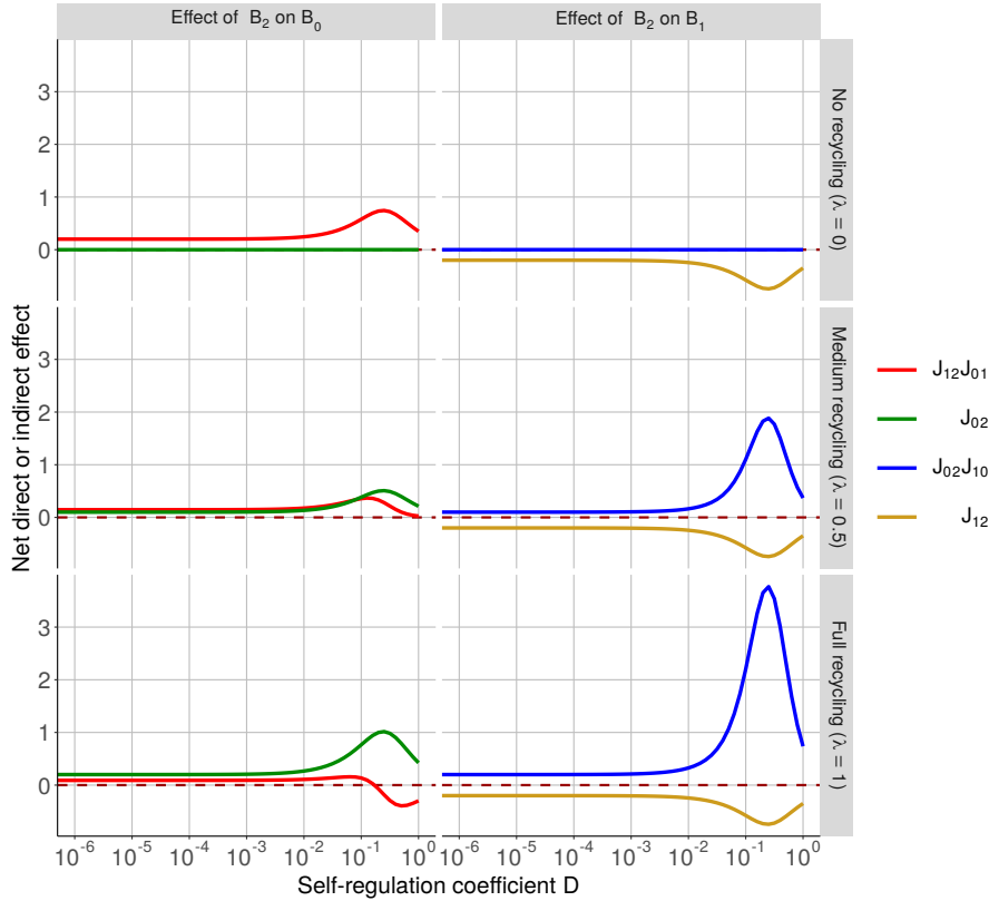
Figure S2-5: Variations in the direct and indirect effects affecting each species depending on recycling efficiency \lambda and self-regulation coefficient D . The effects are calculated from the elements of the Jacobian matrix J for mineral nutrients B_0 and primary producers B_1 . The dashed red line represents the null value of the elements of the Jacobian matrix. J_{12}J_{01} = -a_1B_1 [-a_1B_0 + \lambda(m + 2DB_1) + \lambda(1 - b_2)a_2B_2] ; J_{02} = \lambda(m + 2DB_2) + \lambda(1 - b_2)a_2B_1 ; J_{02}J_{10} = [\lambda(m + 2DB_2) + \lambda(1 - b_2)a_2B_2]a_1B_1 ; J_{12} = -a_2B_1 . The parameter a_2 is equal to 0.4 when D = 0 and to 0.401 when D \neq 0 .
