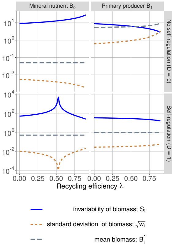
Figure 4: Stability (measured by invariability), standard deviation and biomass of different compartments depending on recycling efficiency \lambda and self-regulation coefficient D in a food chain with a chain length equal to 1 (TL1). Primary producers are perturbed and basal external inputs I are fixed to 0.05.
