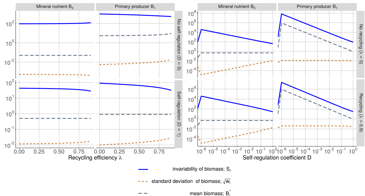
Figure S2-10: Stability of the different compartments depending on A ) recycling efficiency \lambda and B ) self-regulation coefficient D in a food chain with a chain length equal to 1 (TL1). Stability is measured by invariability ( i.e. , inverse of CV), which is the ratio of equilibrium biomass B_i^* to standard deviation \sigma_i . External nutrient input I is fixed to 0.05.
