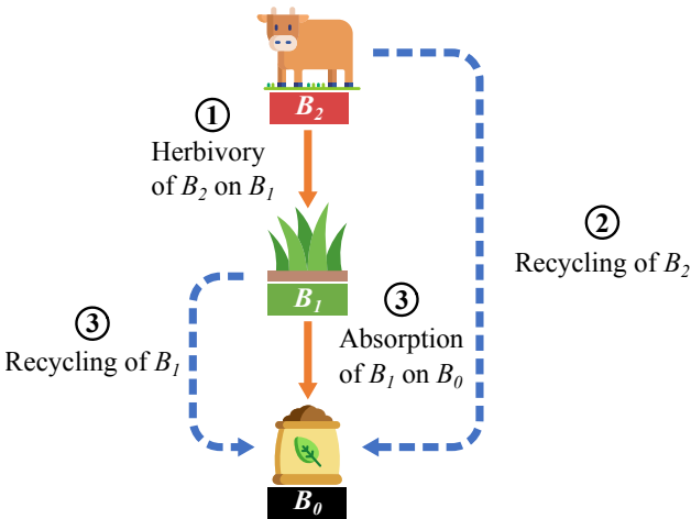
Figure 7: Schematic representing the direct and indirect effects of A ) herbivores on mineral nutrients. Blue arrows represent the positive terms (2) \lambda(m + 2DB_2) + \lambda(1 - b_2)a_2B_1 , (3) \lambda(m + 2DB_1) + \lambda(1 - b_2)a_2B_2 . Orange arrows represent the negative terms (1) -a_2B_1 and (3) -a_1B_0 . Note that the direct effect of B_1 on B_0 (3) is partitioned into its positive and negative terms. B ) Effects of herbivores on primary producers. Blue arrows represent the positive terms (2) \lambda(m + 2DB_2) + \lambda(1 - b_2)a_2B_1 , (3) a_1B_1 . Orange arrows represent the negative terms (1) -a_2B_1 . Note that the effect of nutrient absorption (3) is now positive because it is considered from the perspective of primary producers.
