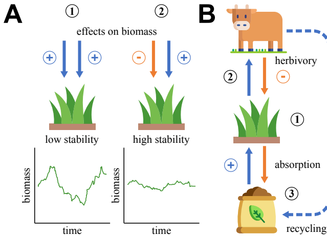
Figure 1: Expected effects on biomass of nutrient cycling feedback loops in a food chain with two trophic levels. A) Net effects on biomass should translate into stability. (1) Effects with the same direction add up and lead to large variations in biomass, thus decreasing stability. (2) Effects with opposite directions cancel each other and lead to small variations in biomass, thus increasing stability. B) In a food chain, this should lead to the stabilisation or the destabilisation of the different trophic levels. Orange arrows represent the negative effect of consumers on their resource while blue solid arrows represent the positive effect of resources on their consumer. Blue dashed arrows represent the positive effect of nutrients recycled by organisms on mineral nutrients. (1) Nutrient cycling generates a positive feedback of herbivores on primary producers due to the increased nutrient availability. This positive effect should offset the negative effect of herbivory and stabilise the dynamics of primary producer biomass. (2) Nutrient cycling generates a positive feedback of herbivores on themselves that should amplify the variations of herbivore biomass and destabilise its dynamics. (3) In a similar way, herbivores have a positive indirect effect on mineral nutrients that adds up to the positive effect of nutrient cycling feedback loop, thus leading to a destabilisation of mineral nutrients.
