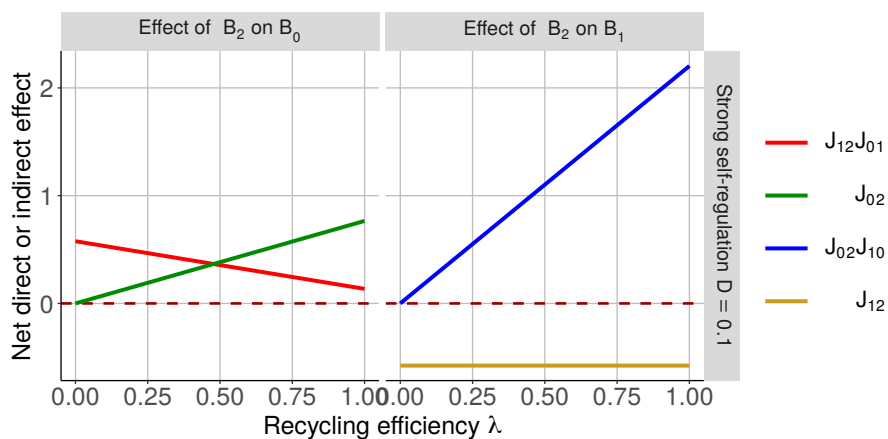
Figure S2-3: Variations in the direct and indirect interaction strengths affecting each species depending on recycling efficiency \lambda and self-regulation coefficient D . Interaction strengths affecting mineral nutrients B_0 and primary producers B_1 are calculated from the elements J_{ij} of the Jacobian matrix. The dashed red line represents null values.
