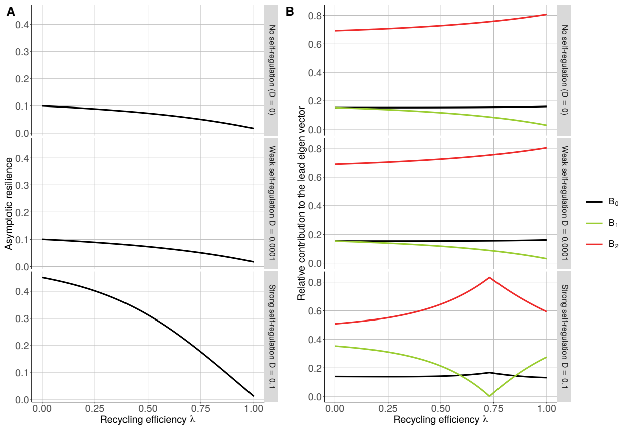
Figure S2-4: Linear stability depending on recycling efficiency \lambda and self-regulation coefficient D in a food chain with a chain length equal to 2 (TL2). A) Asymptotic resilience (opposite of the real part of the lead eigen value of the Jacobian matrix of the system at equilibrium). B) Relative contribution of each compartment to the lead eigen vector.
