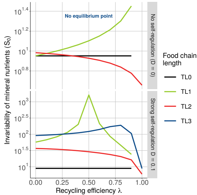
Figure S2-9: Stability of the mineral nutrients B_0 depending on recycling efficiency \lambda and self-regulation coefficient D for various chain lengths. Stability is measured by invariability ( i.e. , inverse of CV), the ratio between equilibrium biomass B_i^* and standard deviation \sigma_i . External nutrient input I is fixed to 0.1 and attack rate a_2 is equal to 0.401.
