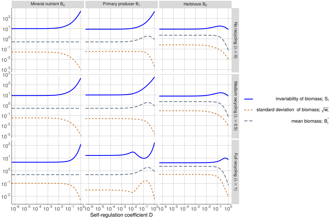
Figure 6: Stability (measured by invariability), standard deviation and biomass of the different compartments depending on recycling efficiency \lambda and self-regulation coefficient D in a food chain with a chain length equal to 2 (TL2). Basal external inputs I are fixed to 0.05, and predation rate a_2 is equal to 0.4 when D = 0 and to 0.401 when D \neq 0 .
