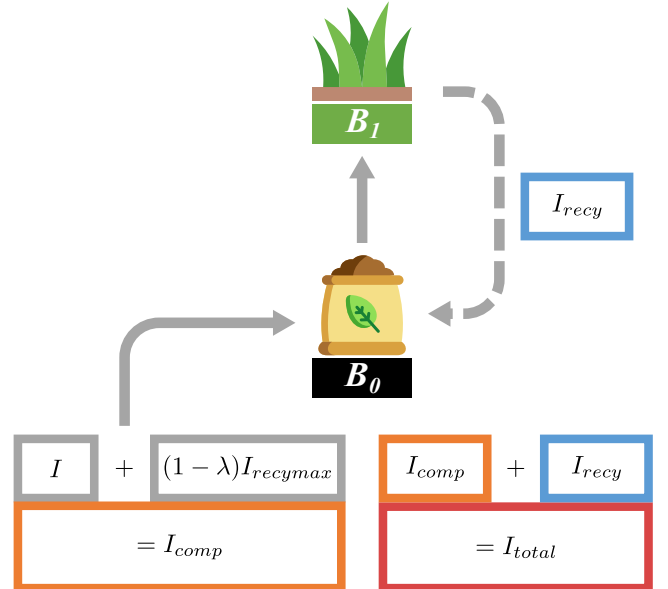
Figure 3: Schematic summarising the different flows of nutrients in the ecosystem. B_0 is the mineral nutrient compartment and B_1 is the primary producer biomass. I is the basal external input, I_{recy} is the quantity of recycled nutrients and I_{recy_{max}} is its value when \lambda = 1 . I_{comp} is the additional external input offsetting fraction 1 - \lambda of nonrecycled nutrients. Thus, I_{total} is constant regardless of the value of \lambda .
