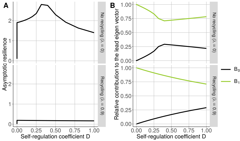
Figure S2-8: Linear stability depending on recycling efficiency \lambda and self-regulation coefficient D in a food chain with a chain length equal to 1 (TL1). A) Asymptotic resilience (opposite of the real part of the lead eigen value of the Jacobian matrix of the system at equilibrium). B) Relative contribution of each compartment to the lead eigen vector.
