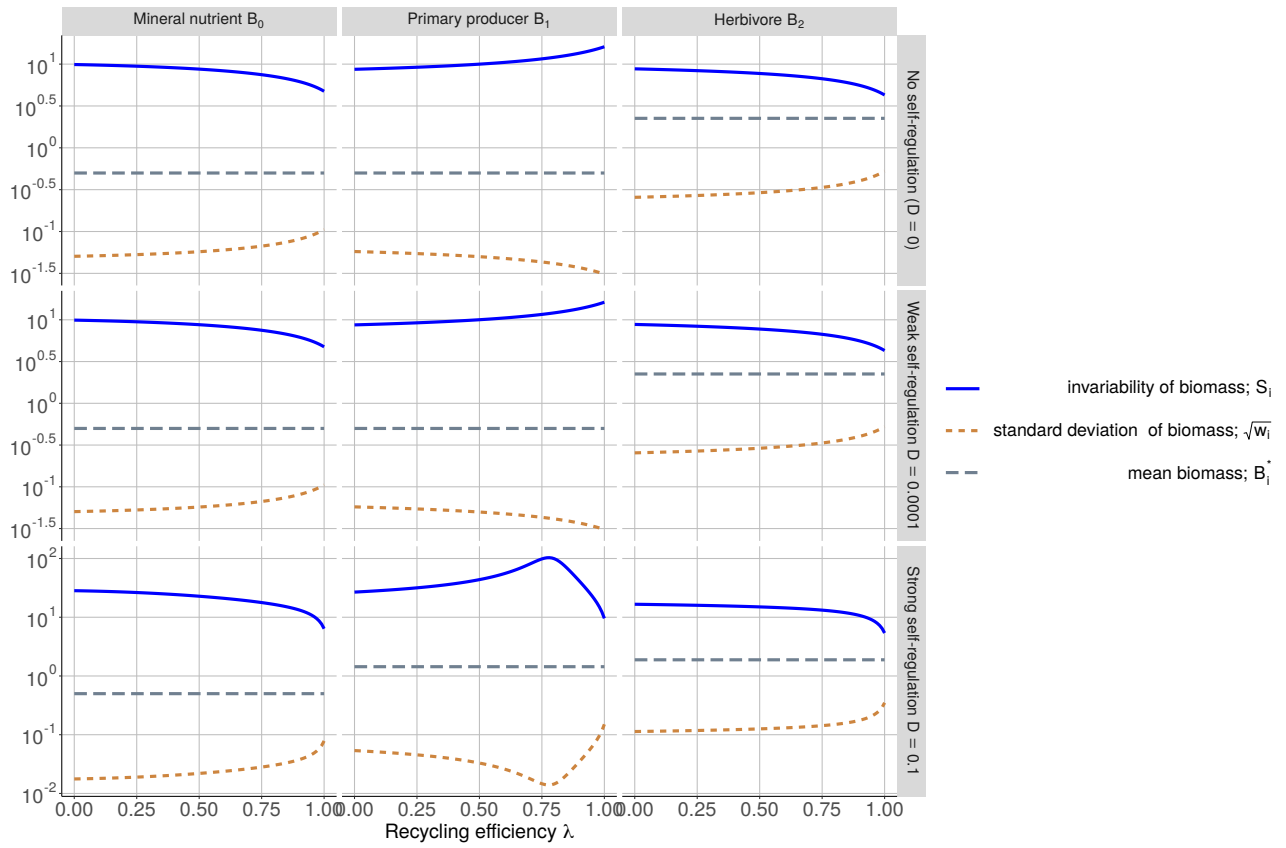
Figure S2-2: Stability of different compartments depending on recycling efficiency \lambda and self-regulation coefficient D in a food chain with a chain length equal to 2 (TL2). Herbivores are perturbed, basal external inputs I are fixed to 0.05, and predation rate a_2 is equal to 0.4 when D = 0 and to 0.401 when D \neq 0 .
