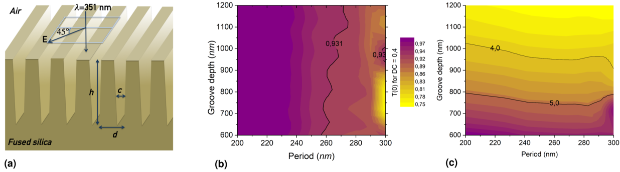
Fig. 1. Numerical design of a silica-based UV quarter-wave plate. (a) Schematic representation of the periodically nanostructured glass with groove depth h and groove width at mid-height c . The substrate is made of glass with an index of refraction of 1.47605, and the superstrate is made of air. The incoming beam has a normal incidence, and a linear polarization with an electric field oriented at 45^\circ from the orientation of the grooves. Wavelength is \lambda = 351 nm. (b) Transmission efficiency T^0 in the zeroth order averaged over both polarizations T^0 = \frac{1}{2}[T_{TE}^0 + T_{TM}^0] with respect to the period d and the groove depth for a duty cycle DC = 0.4 ; high transmission, larger than 93%, is obtained for periods smaller than 260 nm. (c) Difference of phase \Delta\phi induced by the metamaterial wave plate expressed in terms of \lambda/x , by plotting x = 2\pi/\Delta\phi with respect to the period d and duty cycle DC for a period of 260 nm. \Delta\phi is obtained by calculating the difference of phase between the transmitted electric field in the zeroth order parallel (TE) or perpendicular (TM) to the fast axis (parallel to the grooves). Significant beam smoothing requires at least a \lambda/5 and ideally a \lambda/4 metamaterial wave plate; this area of interest is delimited in the figure.
