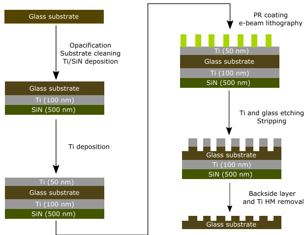
Fig. 3. Metamaterial wave plate process flow. The first step consists of opacifying the back side of the substrate due to the deposition of Ti and SiN layers. A Ti layer is then deposited on the front side. A photo-resistive layer is coated on this latter layer and written by electron beam lithography. A two-step etching process is then used to obtain the final nanostructure.
