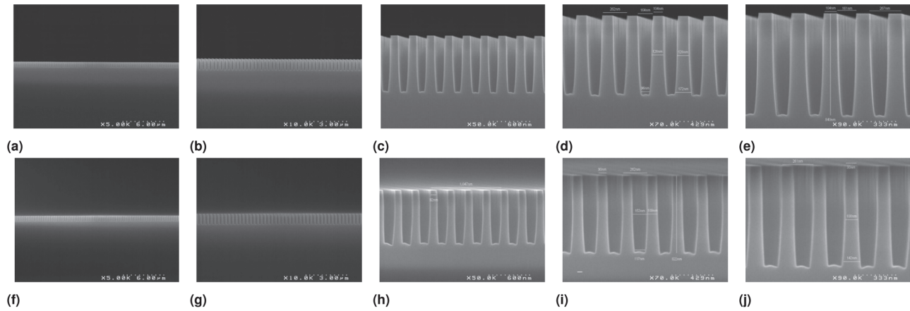
Fig. 4. SEM cross-section images at different magnifications on the center (top) and edge (bottom) of the clear aperture of the final metamaterial wave plate. The groove depths range between 820 nm and 840 nm, sidewall angle is about 87.5^\circ , and line and space widths are detailed in Table 1.
