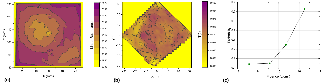
Fig. 5. Optical and laser damage characterization results. (a) Spatial distribution of the experimental retardance of the metamaterial wave plate. Measurement at normal incidence at the wavelength of 355 nm. A mean retardance of 70.2 nm is obtained with good uniformity. (b) Spatial distribution of the specular transmission T^0 at normal incidence at the wavelength of 351 nm. A mean diffraction efficiency of 0.9159 is obtained. (c) Laser induced damage probability measurement at the wavelength of 355 nm. Experiments are carried out in normal incidence with a pulse duration of 2.5 ns and a nanostructure placed on the front side with respect to the testing beam; a damage threshold of 13 \text{ J}/\text{cm}^2 is measured.
