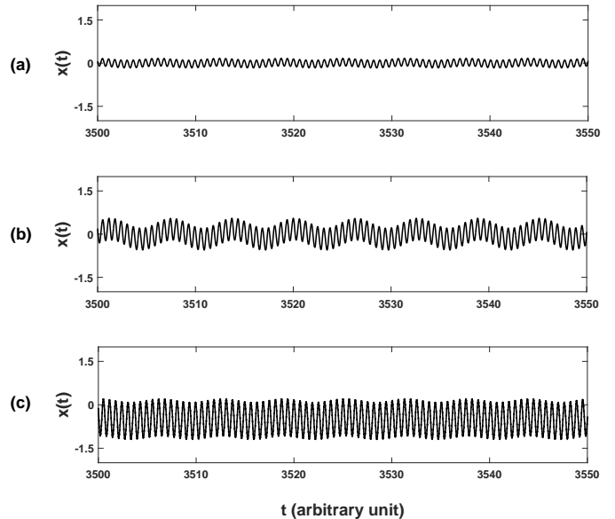
Figure 3: Typical time series of the Chua model experiencing the truncated sinusoidal force defined by eq. (4) and driven by the excitation of eq. (8). The chronograms of x have been obtained by increasing the perturbation amplitude starting from B = 0 with step \Delta B = 0.01 until (a) B = 1.5 , (b) B = 4.13 , (c) B = 6.8 . Model parameters: n = 1 , k = 1 , V_0 = \frac{\pi}{32} , \alpha = 6 , \beta = 16 , b = 0.1 , \omega_1 = 1 , \Omega = 10\omega_1 , numerical time step \Delta t = 0.0015 .
