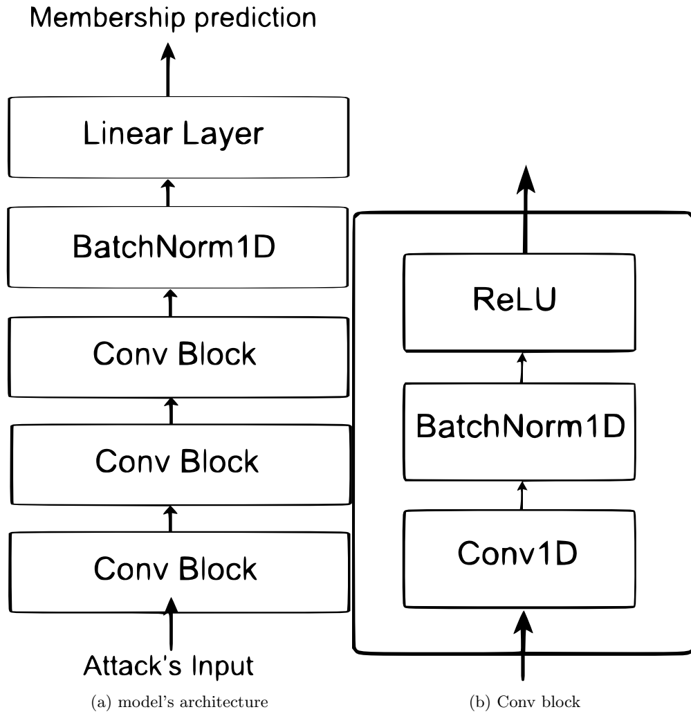
Figure 4: The architecture of the attack model consisting of three convolution blocks, one-dimensional batch normalization and a final linear layer with binary membership prediction.
